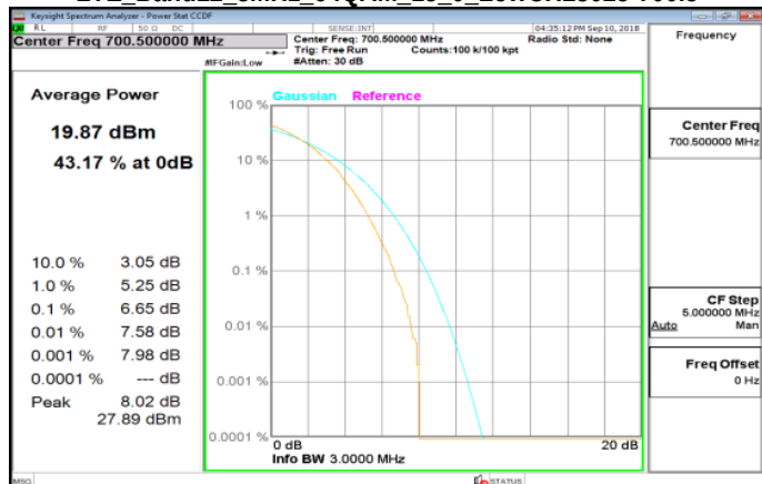
LTE_Band12_3MHz_64QAM_15_0_LowCH23025-700.5
