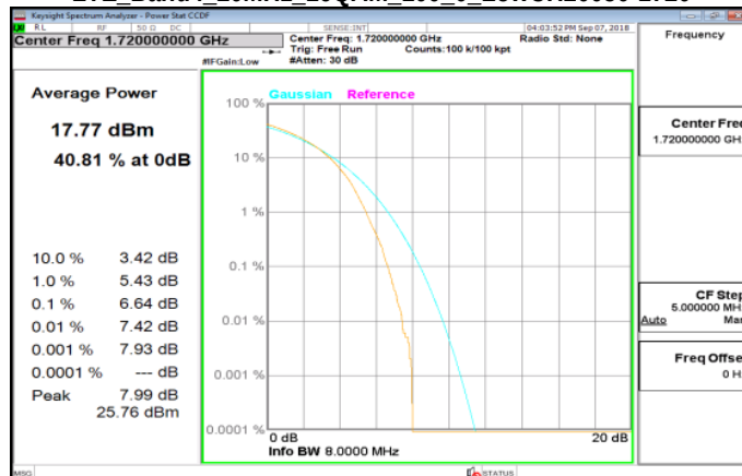
LTE_Band4_20MHz_16QAM_100_0_LowCH20050-1720
