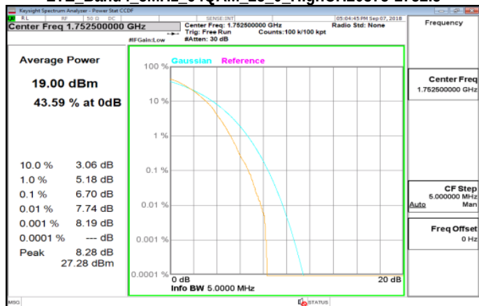
LTE_Band4_5MHz_64QAM_25_0_HighCH20375-1752.5
