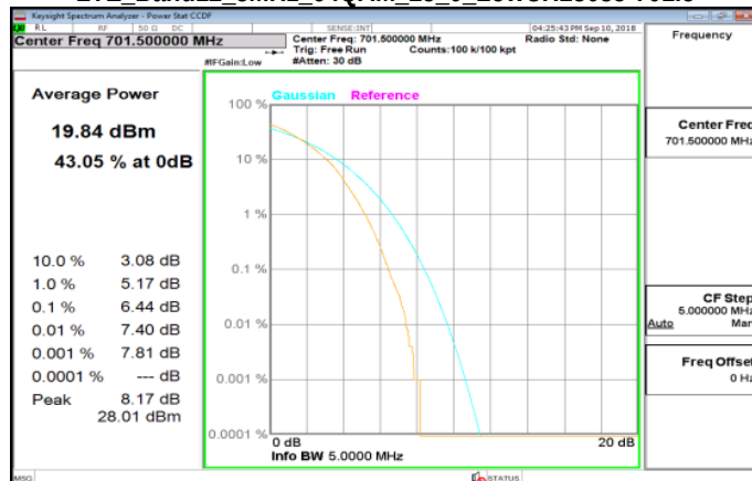
LTE_Band12_5MHz_64QAM_25_0_LowCH23035-701.5
