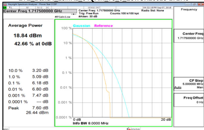
LTE_Band4_15MHz_64QAM_75_0_LowCH20025-1717.5
