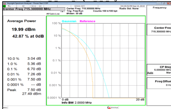
LTE_Band12_1_4MHz_64QAM_6_0_HighCH23173-715.3
