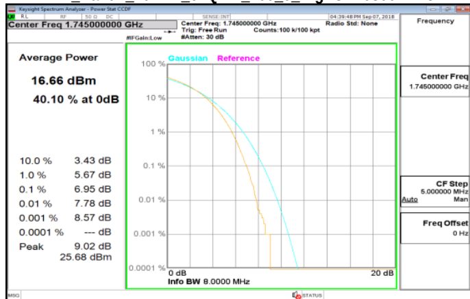
LTE_Band4_20MHz_64QAM_100_0_HighCH20300-1745
