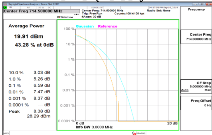
LTE_Band12_3MHz_64QAM_15_0_HighCH23165-714.5
