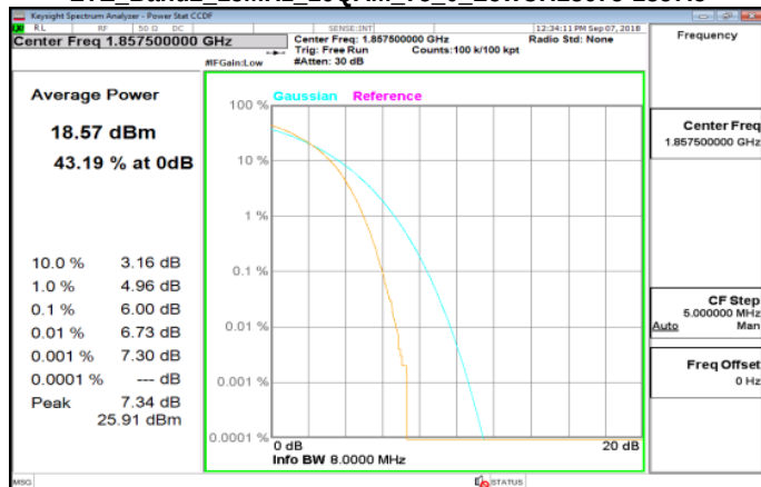
LTE_Band2_15MHz_64QAM_75_0_LowCH18675-1857.5
