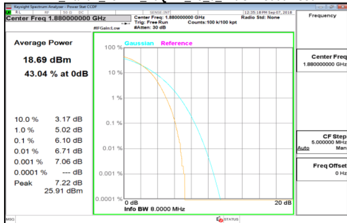
LTE_Band2_15MHz_16QAM_75_0_MidCH18900-1880
