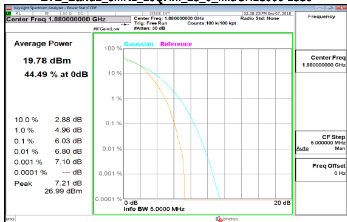
LTE_Band2_5MHz_16QAM_25_0_MidCH18900-1880
