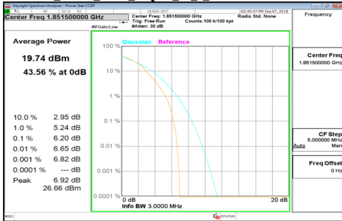
LTE_Band2_3MHz_16QAM_15_0_LowCH18615-1851.5
