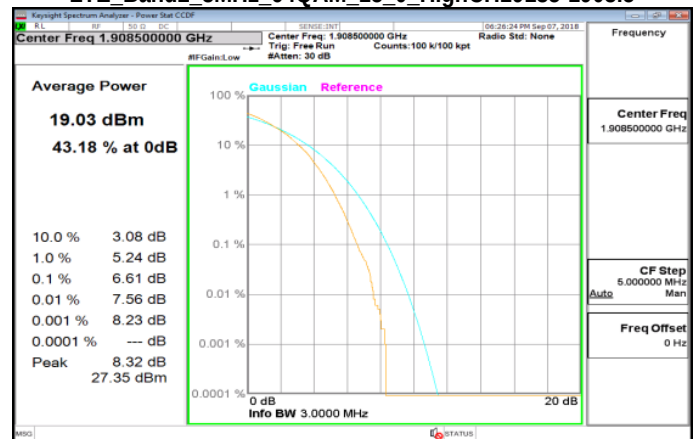
LTE_Band2_3MHz_64QAM_15_0_HighCH19185-1908.5
