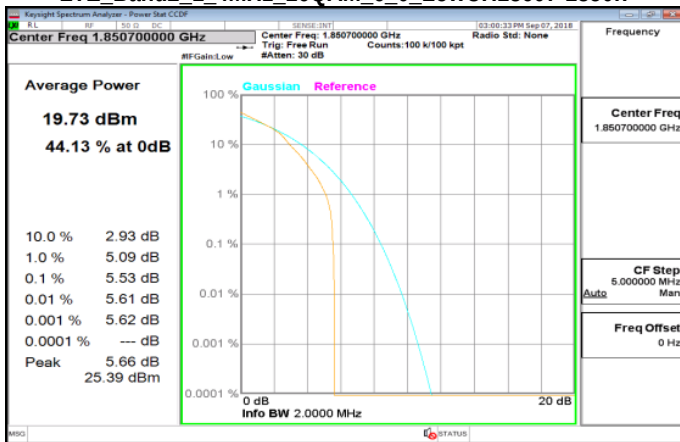
LTE_Band2_1_4MHz_64QAM_6_0_LowCH18607-1850.7
