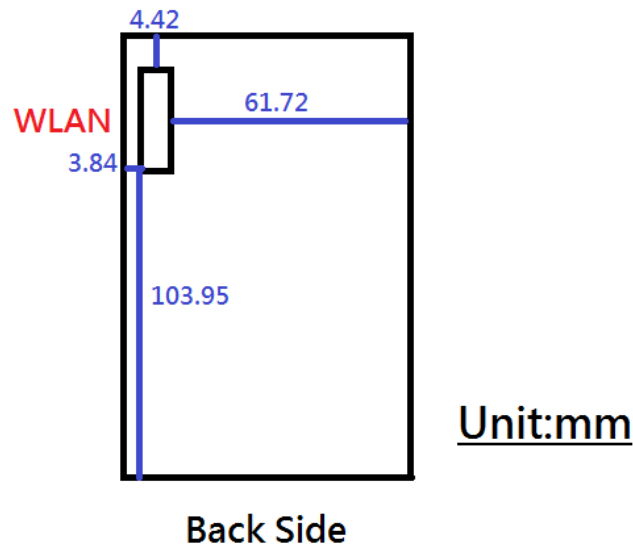
Fig.21 Antenna position of EUT
