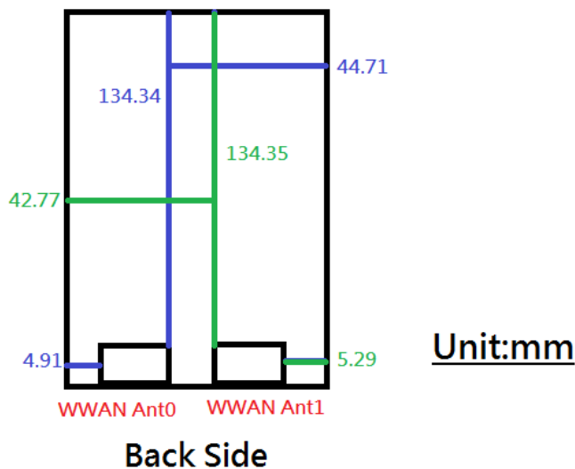
Fig.22 Antenna position of EUT
