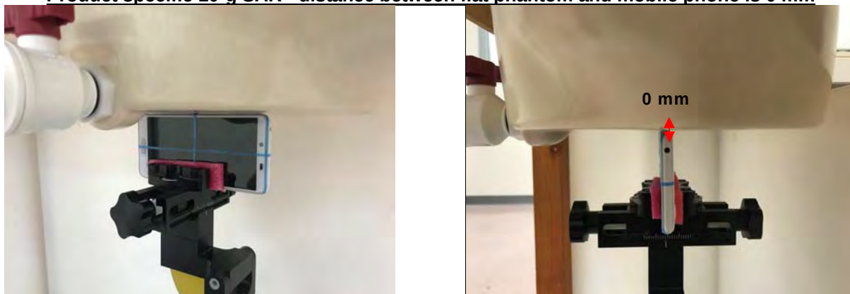
Fig.18 EUT Left side to flat phantom
