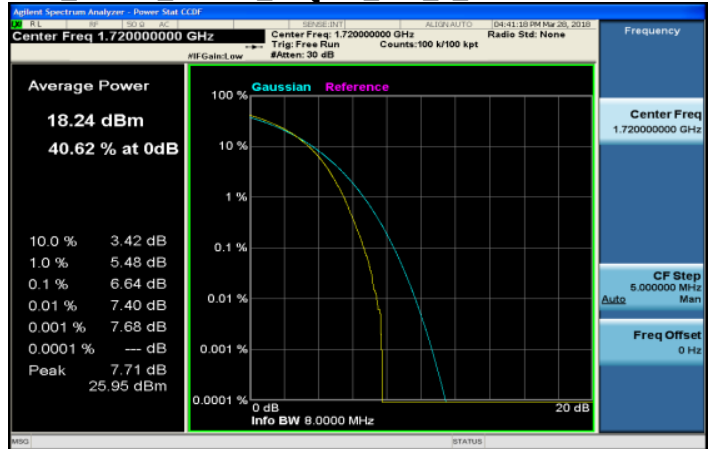
LTE_Band4_20MHz_64QAM_100_0_LowCH20050-1720
