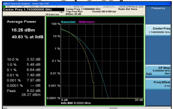
LTE_Band4_20MHz_64QAM_100_0_HighCH20300-1745
