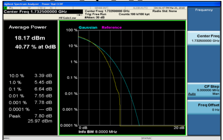
LTE_Band4_20MHz_64QAM_100_0_MidCH20175-1732.5
