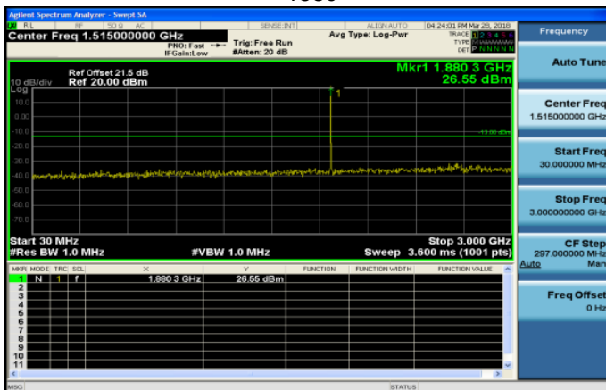
30MHz~3GHz_Band2_1_4MHz_QPSK_1_0_MidCH18900 -1880
