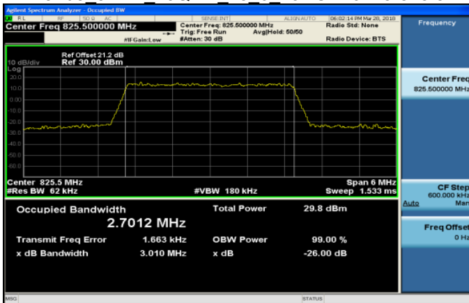
Band5 3MHz 16QAM 15_0 LowCH20415-825.5
