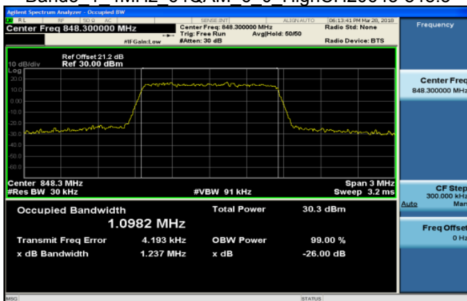
Band5 1 4MHz 64QAM 6 0 HighCH20643-848.3
