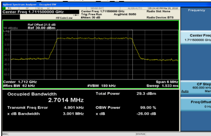
Band4 3MHz 16QAM 15 0 LowCH19965-1711.5
