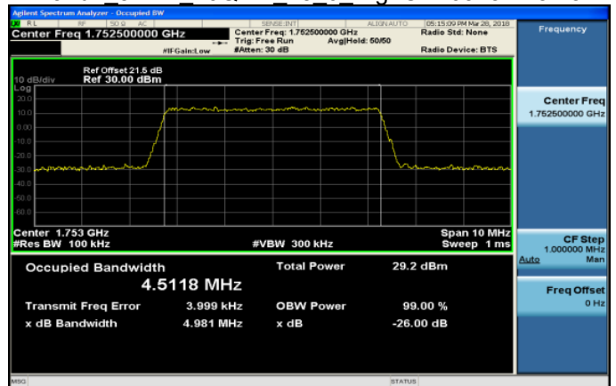
Band4 5MHz 16QAM 25 0 HighCH20375-1752.5
