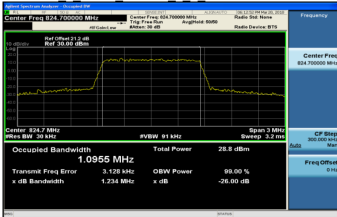
Band5 1 4MHz 64QAM 6 0 LowCH20407-824.7
