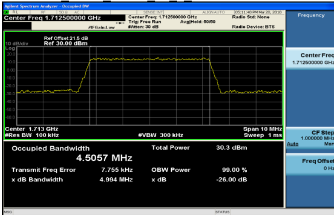
Band4 5MHz QPSK 25 0 LowCH19975-1712.5
