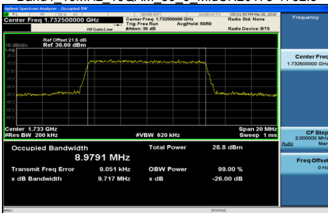
Band4 10MHz 16QAM 50 0 MidCH20175-1732.5
