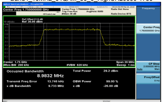
Band4 10MHz 64QAM 50 0 HighCH20350-1750
