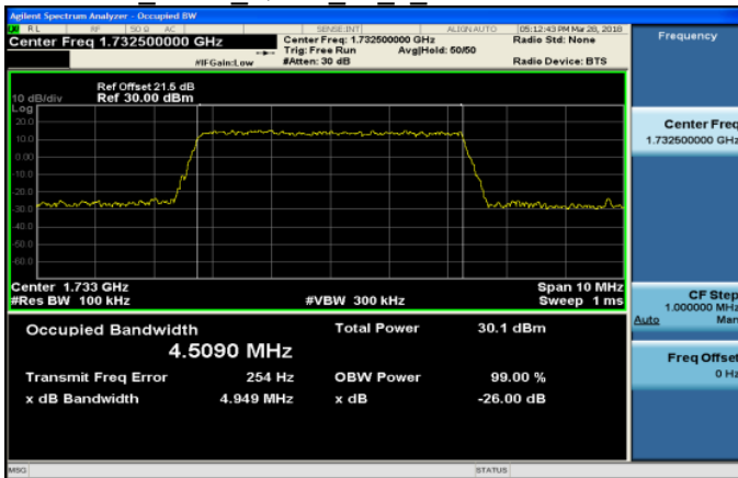
Band4 5MHz QPSK 25 0 MidCH20175-1732.5
