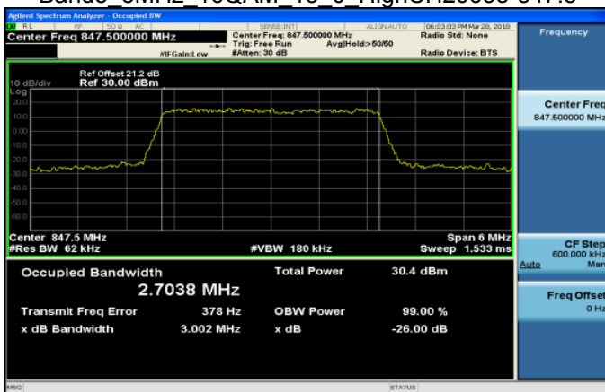
Band5 3MHz 16QAM 15_0 HighCH20635-847.5
