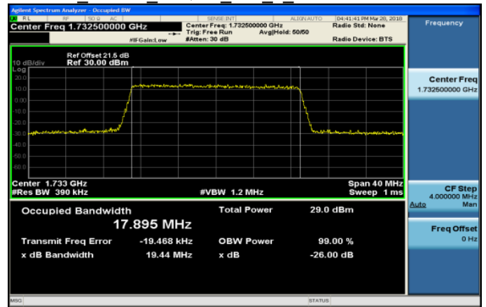
Band4 20MHz 64QAM 100 0 MidCH20175-1732.5
