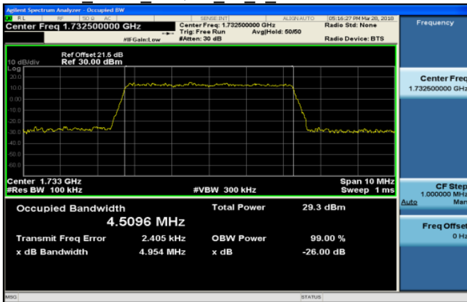
Band4 5MHz 64QAM 25 0 MidCH20175-1732.5
