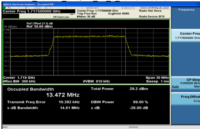
Band4 15MHz 64QAM 75 0 LowCH20025-1717.5
