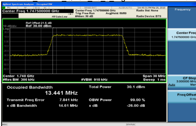
Band4 15MHz QPSK 75 0 HighCH20325-1747.5
