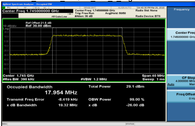
Band4 20MHz 16QAM 100 0 HighCH20300-1745
