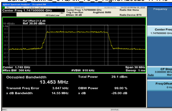
Band4 15MHz 64QAM 75 0 HighCH20325-1747.5
