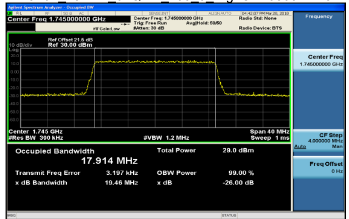
Band4 20MHz 64QAM 100 0 HighCH20300-1745
