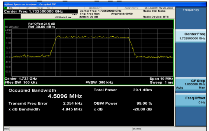
Band4 5MHz 16QAM 25 0 MidCH20175-1732.5
