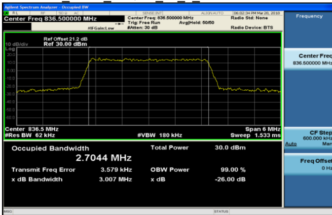
Band5 3MHz 16QAM 15_0 MidCH20525-836.5
