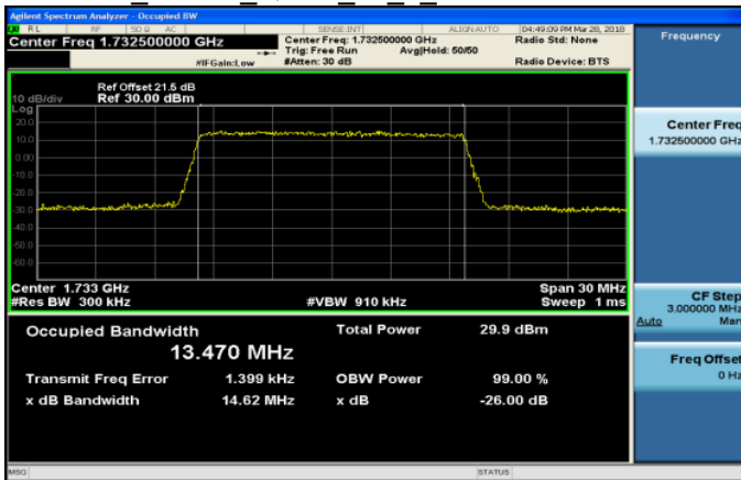
Band4 15MHz QPSK 75 0 MidCH20175-1732.5
