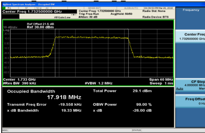
Band4 20MHz 16QAM 100 0 MidCH20175-1732.5
