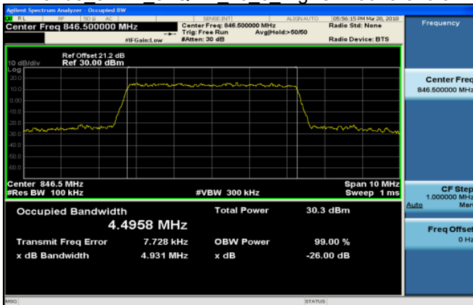
Band5 5MHz 64QAM 25 0 HighCH20625-846.5
