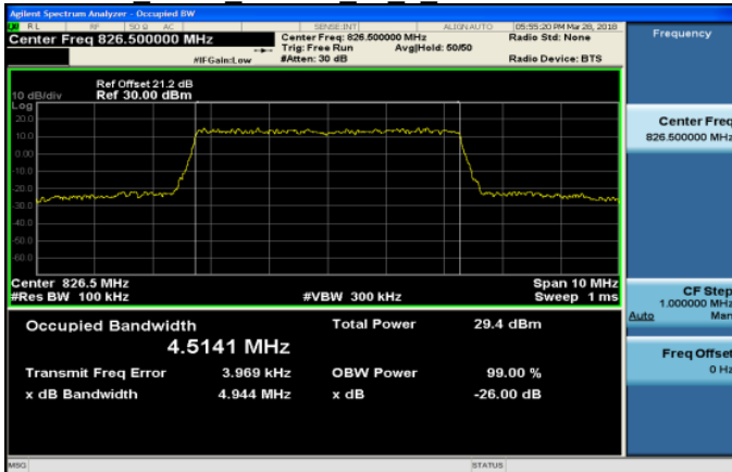
Band5 5MHz 64QAM 25 0 LowCH20425-826.5
