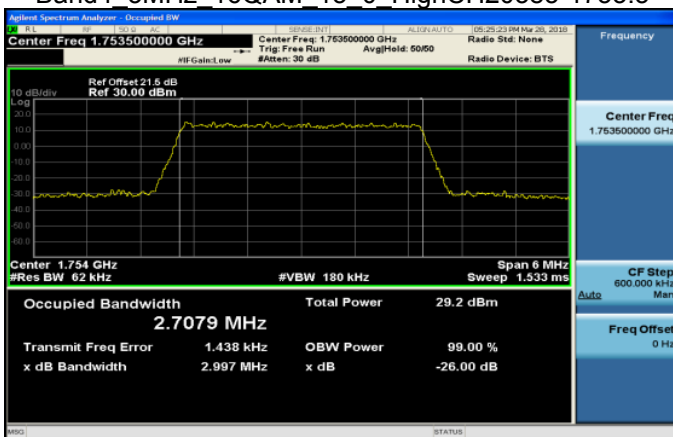
Band4 3MHz 16QAM 15 0 HighCH20385-1753.5
