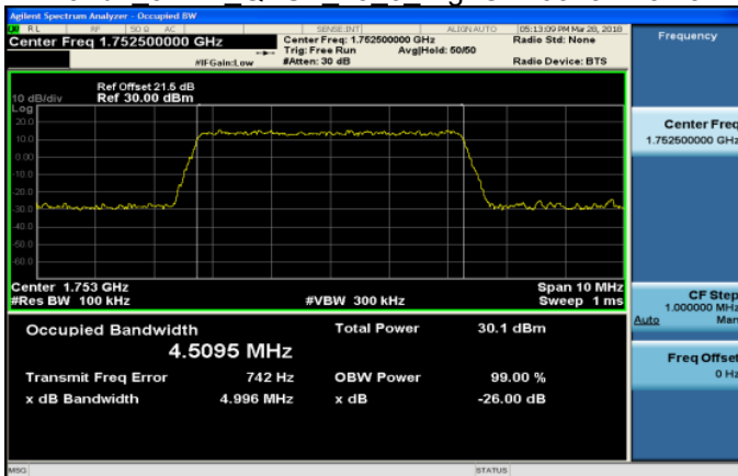
Band4 5MHz QPSK 25 0 HighCH20375-1752.5
