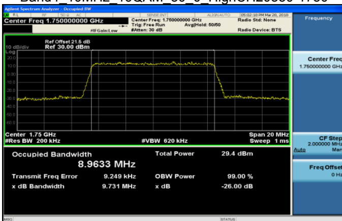
Band4 10MHz 16QAM 50 0 HighCH20350-1750
