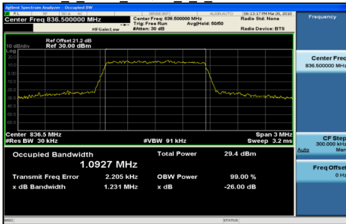
Band5 1 4MHz 64QAM 6 0 MidCH20525-836.5
