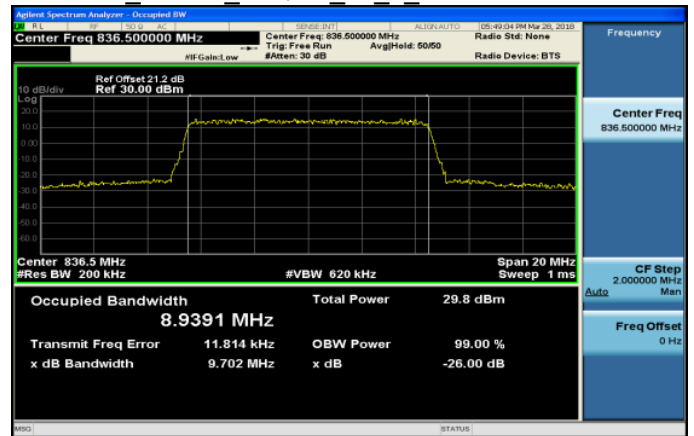
Band5 10MHz 64QAM 50 0 MidCH20525-836.5
