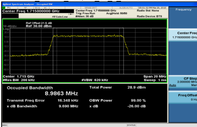
Band4 10MHz 16QAM 50 0 LowCH20000-1715
