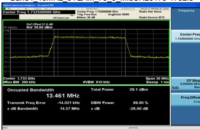
Band4 15MHz 64QAM 75 0 MidCH20175-1732.5
