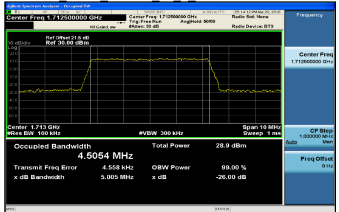
Band4 5MHz 16QAM 25 0 LowCH19975-1712.5
