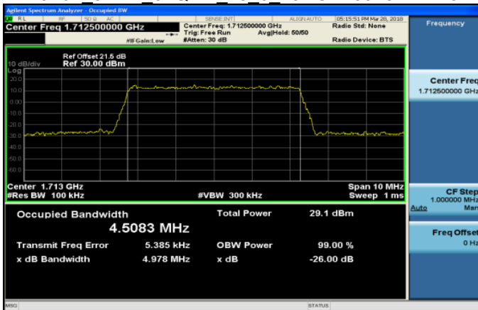
Band4 5MHz 64QAM 25 0 LowCH19975-1712.5
