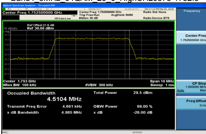
Band4 5MHz 64QAM 25 0 HighCH20375-1752.5
