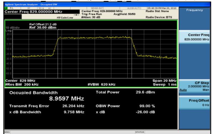
Band5 10MHz 64QAM 50 0 LowCH20450-829
