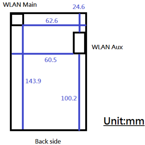
Fig.22 Antenna position of EUT
