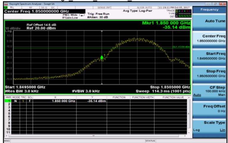
Band Edge GPRS 1900MHz LowCH512-1850.2
