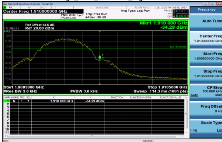
Band Edge GSM 1900MHz HighCH810-1909.8
