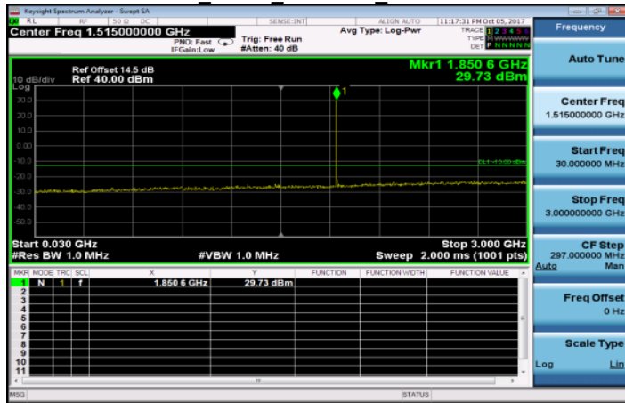
30MHz~3GHz GPRS 1900MHz LowCH512-1850.2
