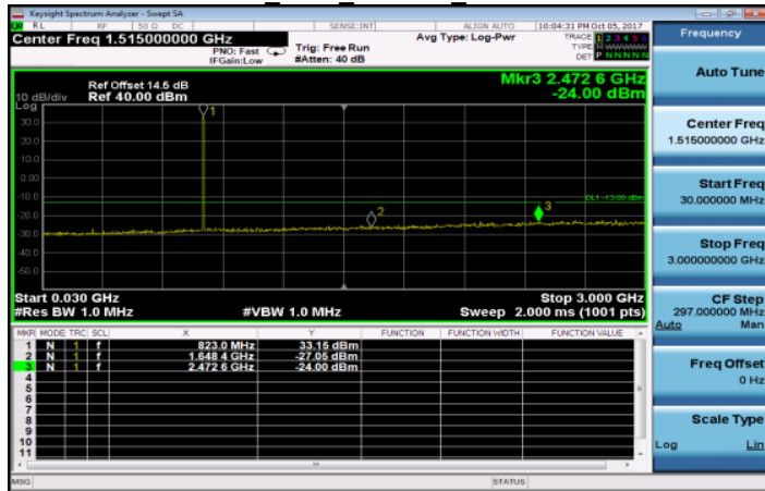
30MHz~3GHz GSM 850MHz LowCH128-824.2
