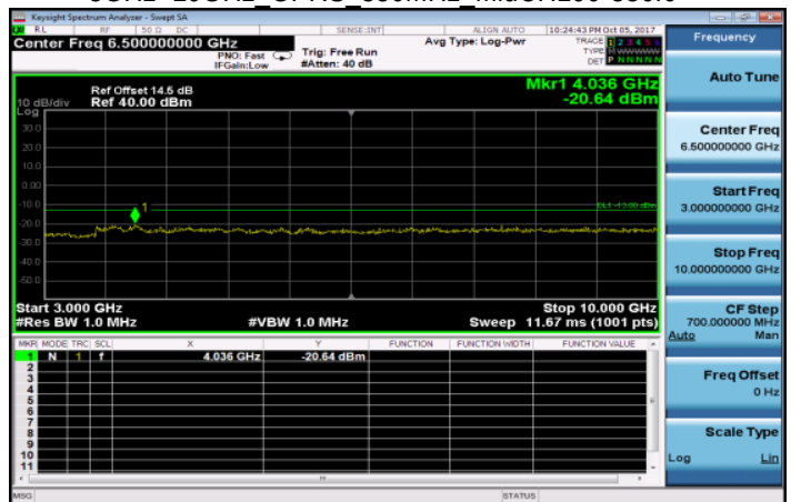
3GHz~10GHz GPRS 850MHz MidCH190-836.6
