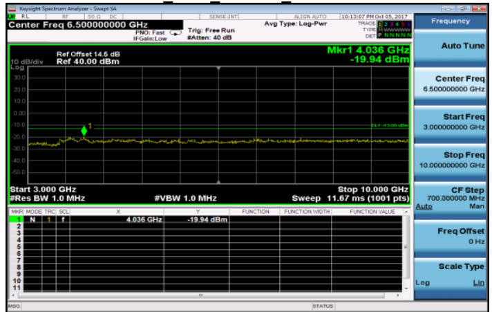
3GHz~10GHz GSM 850MHz MidCH190-836.6
