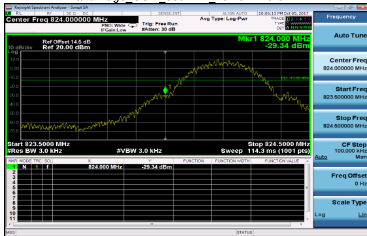
Band Edge GSM 850MHz LowCH128-824.2
