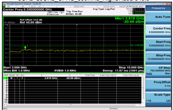
3GHz~10GHz GPRS 850MHz HighCH251-848.8
