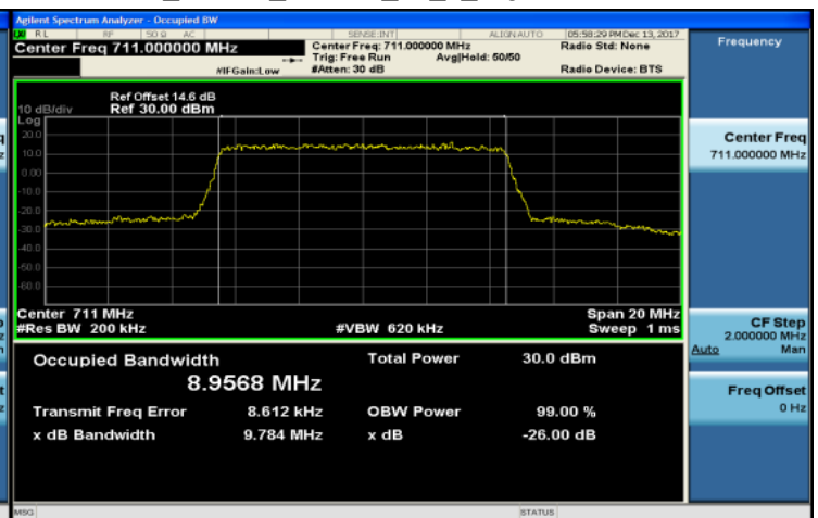
Band12_10MHz_16QAM_50_0_HighCH23130-711
