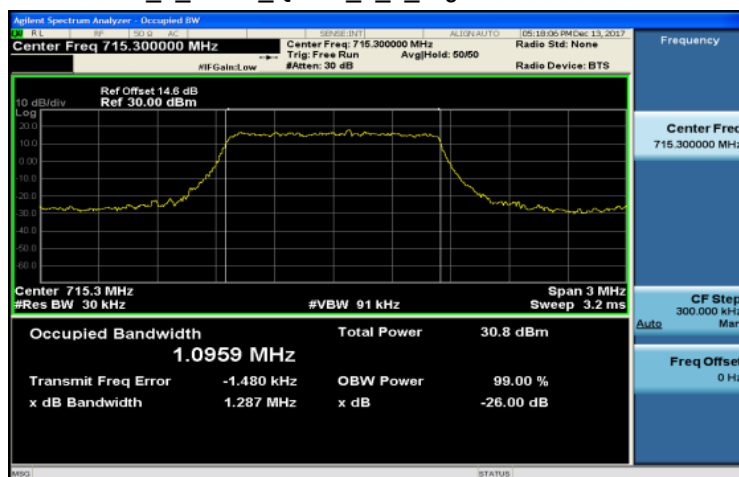
Band12_1_4MHz_QPSK_6_0_HighCH23173-715.3
