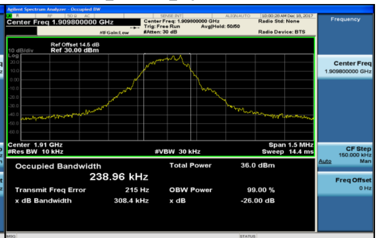
GPRS_1900MHz_HighCH810-1909.8
