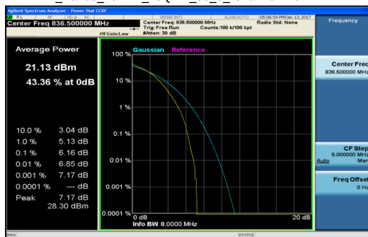
LTE_Band5_10MHz_16QAM_50_0_Channel Mid
