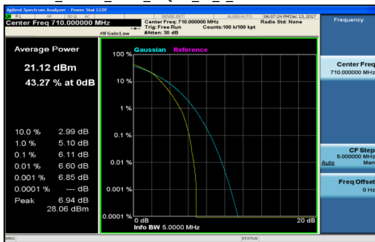
LTE_Band17_5MHz_16QAM_25_0_Channel Mid
