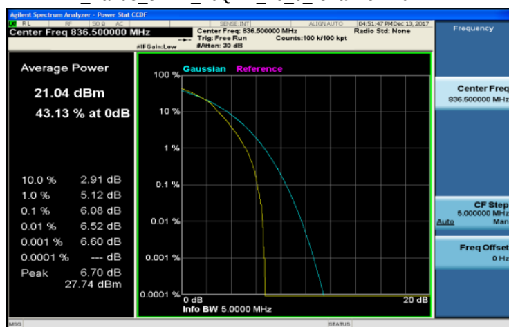
LTE_Band5_5MHz_16QAM_25_0_Channel Mid
