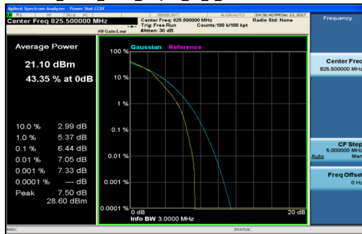
LTE_Band5_3MHz_16QAM_15_0_Channel Low
