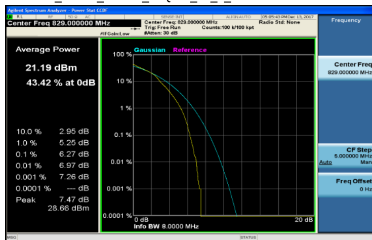
LTE_Band5_10MHz_16QAM_50_0_Channel Low
