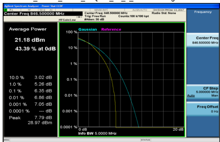
LTE_Band5_5MHz_16QAM_25_0_Channel High
