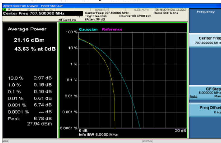
LTE_Band12_5MHz_16QAM_25_0_Channel Mid
