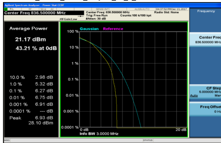
LTE_Band5_3MHz_16QAM_15_0_Channel Mid
