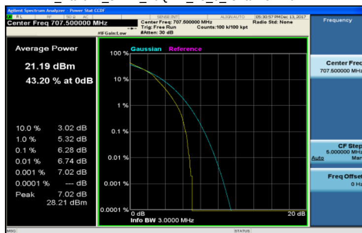
LTE_Band12_3MHz_16QAM_15_0_Channel Mid
