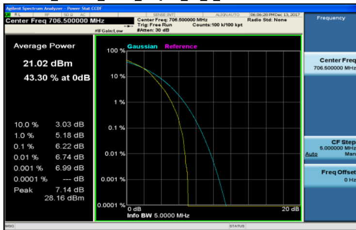
LTE_Band17_5MHz_16QAM_25_0_Channel Low
