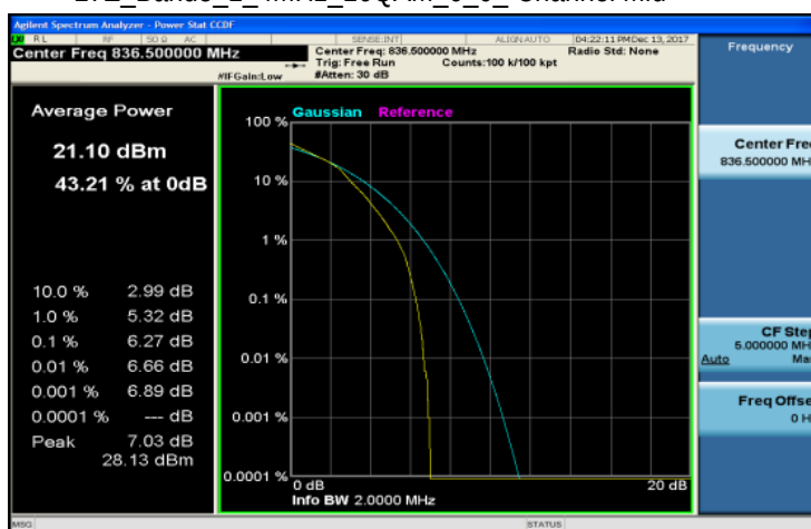
LTE_Band5_1_4MHz_16QAM_6_0_Channel Mid
