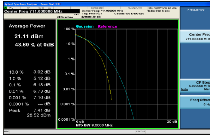
LTE_Band17_10MHz_16QAM_50_0_Channel High
