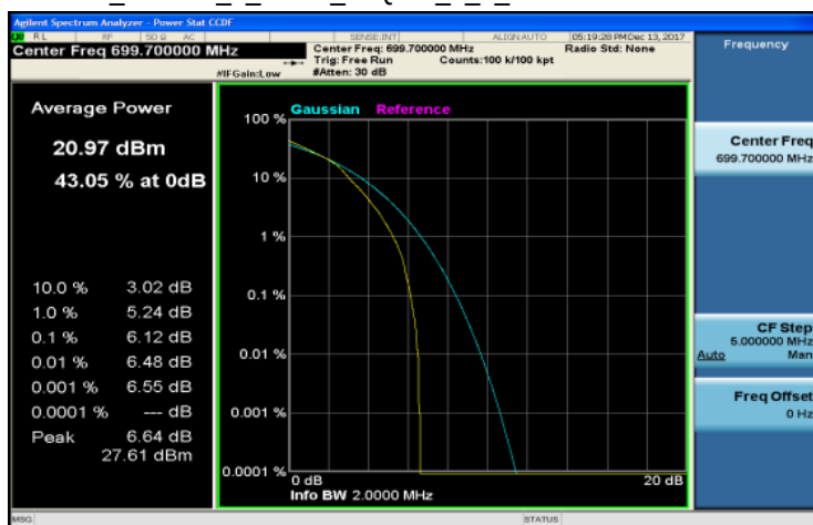
LTE_Band12_1_4MHz_16QAM_6_0_Channel Low
