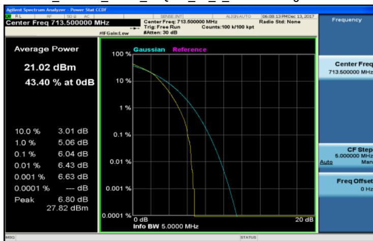
LTE_Band17_5MHz_16QAM_25_0_Channel High
