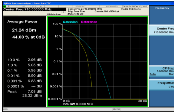
LTE_Band17_10MHz_16QAM_50_0_Channel Mid
