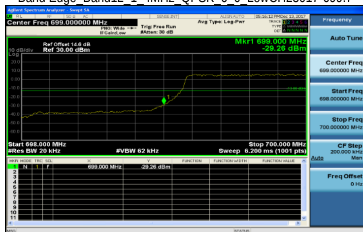
Band Edge Band12 1 4MHz QPSK 6 0 LowCH23017-699.7
