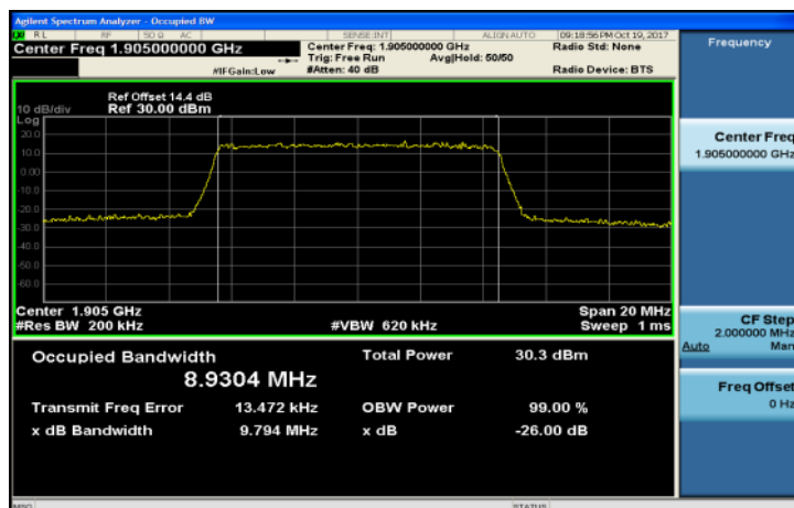
Band2_10MHz_16QAM_50_0_HighCH19150-1905
