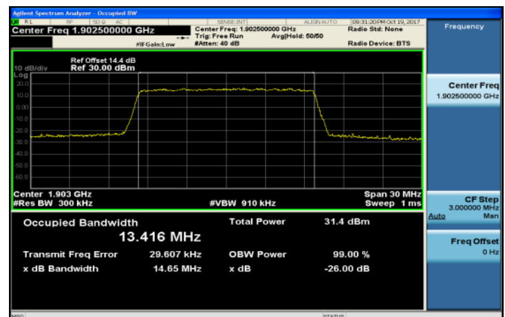
Band2_15MHz_QPSK_75_0_HighCH19125-1902.5
