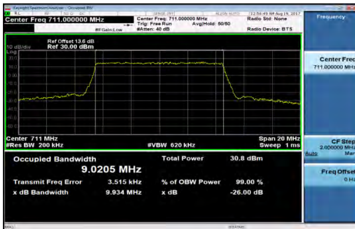
Band12_10MHz_QPSK_50_0_HighCH23130-711
