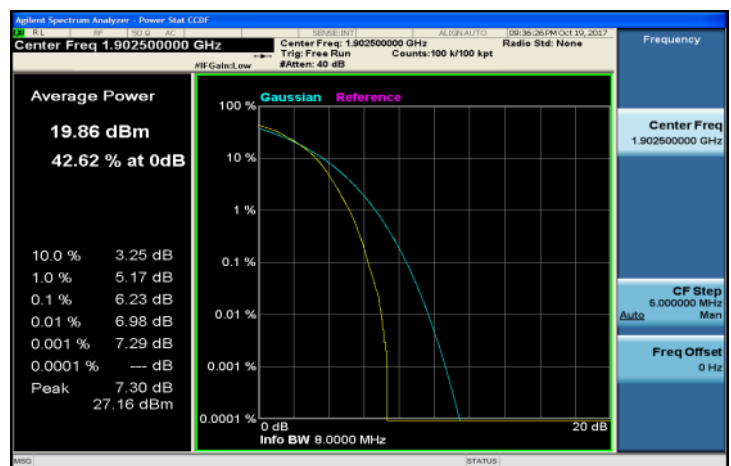
LTE_Band2_15MHz_16QAM_75_0_HighCH19125-1902.5
