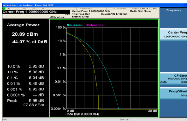
LTE_Band2_10MHz_16QAM_50_0_HighCH19150-1905
