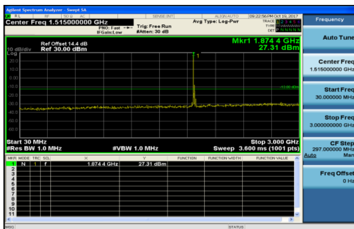
30MHz~3GHz_Band2_15MHz_QPSK_1_0_MidCH18900-1880
