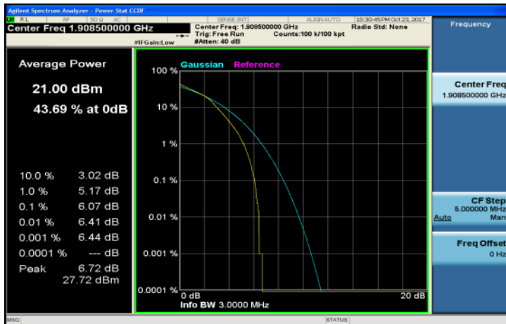
LTE_Band2_3MHz_QPSK_15_0_HighCH19185-1908.5
