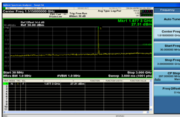
30MHz~3GHz_Band2_10MHz_QPSK_1_0_MidCH18900-1880
