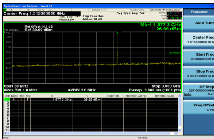
30MHz~3GHz_Band2_5MHz_QPSK_1_0_MidCH18900-1880
