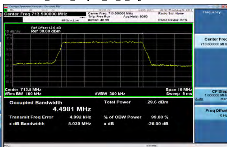
Band17_5MHz_16QAM_25_0_HighCH23825-713.5
