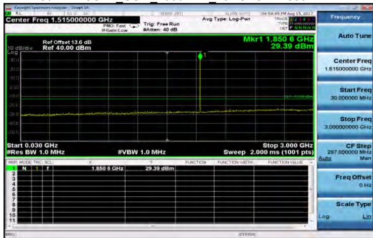
30MHz~3GHz GSM 1900MHz LowCH512-1850.2
