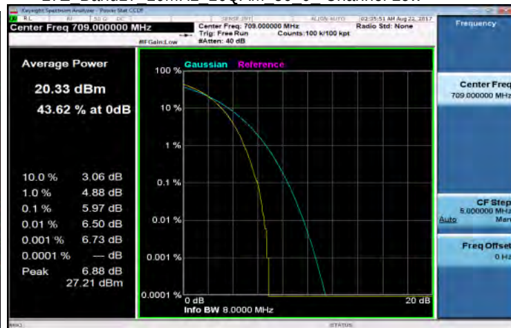
LTE_Band17_10MHz_16QAM_50_0_Channel Low
