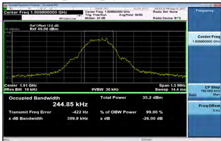
GPRS_1900MHz_HighCH810-1909.8
