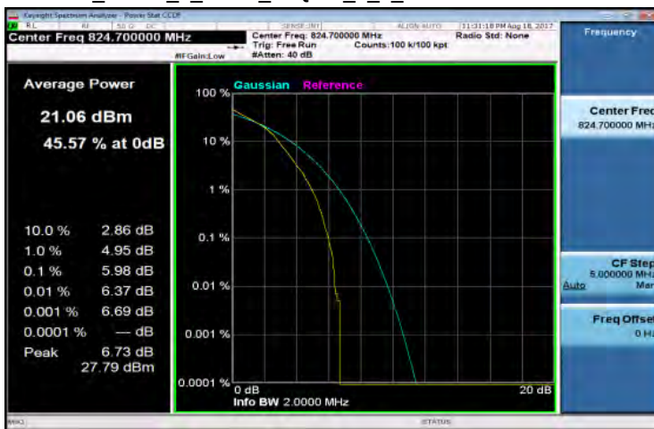
LTE_Band5_1_4MHz_16QAM_6_0_Channel Low
