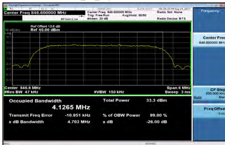
WCDMA_B5_HighCH4233-846.6
