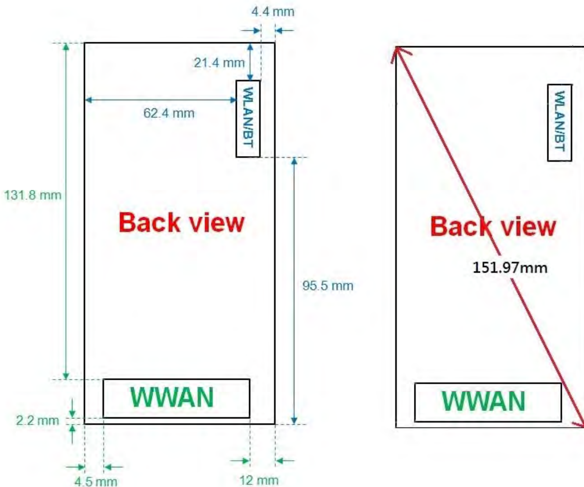
Fig.17 Antenna position of EUT
