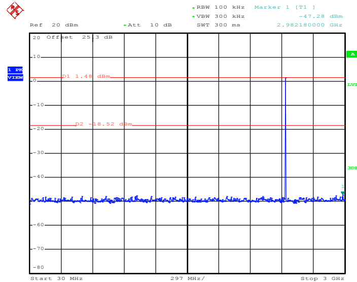
2Mbps CSE Plot on Ch 39 between 30MHz ~ 3 GHz
