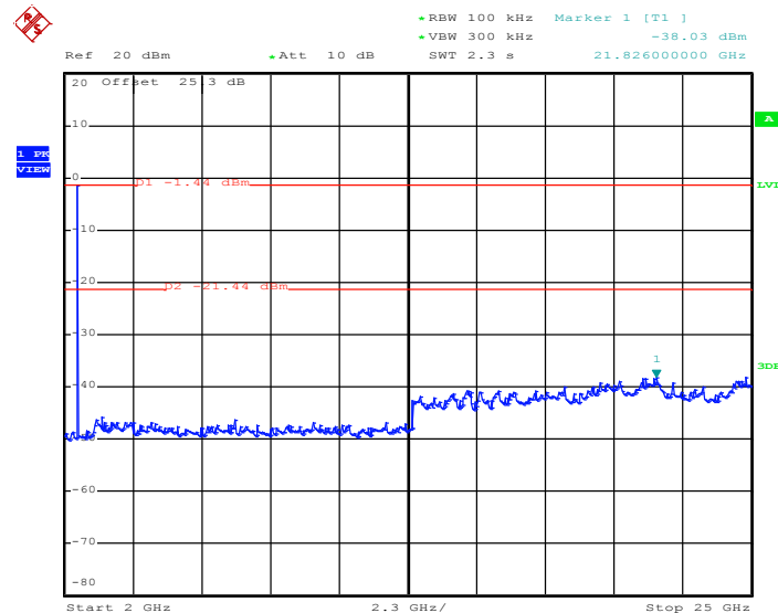
2Mbps CSE Plot on Ch 39 between 2 GHz ~ 25 GHz
