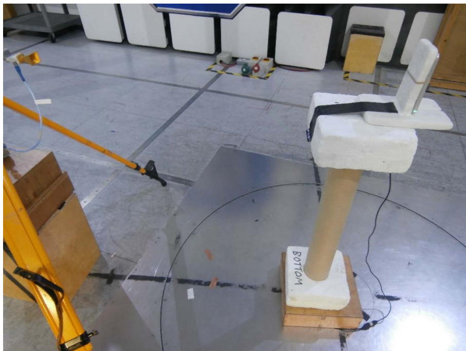
FCC Part 15.247 Radiated Emissions 18 GHz to 25 GHz
