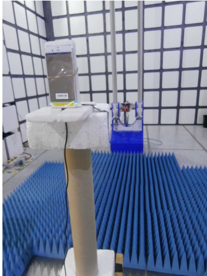
FCC Part 15.407 Radiated Emissions 1 GHz to 18 GHz
