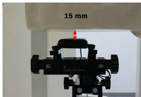
Fig.9 EUT back side with headset to flat phantom
