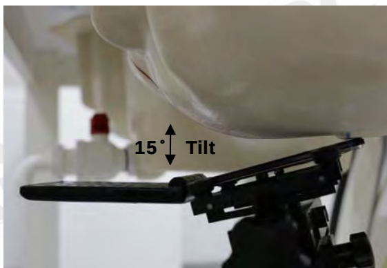
Fig.6 Left Head Section / Ear-Tilt Position(15°)
