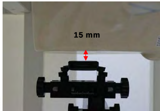
Fig.7 EUT front to flat phantom
