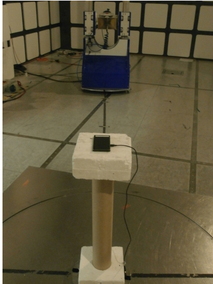
FCC Part 15.247 Radiated Emissions 1 GHz to 18 GHz
