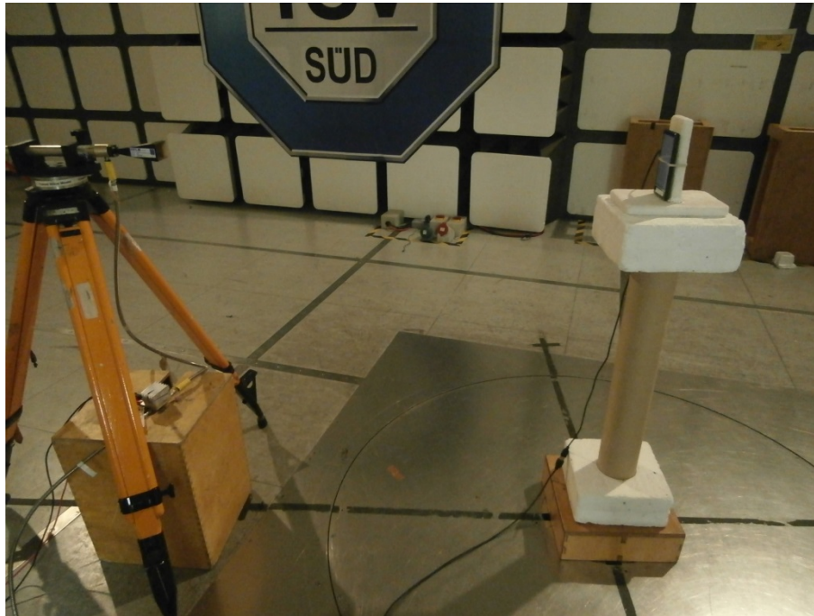
FCC Part 15.407 Radiated Emissions 18 GHz to 40 GHz
