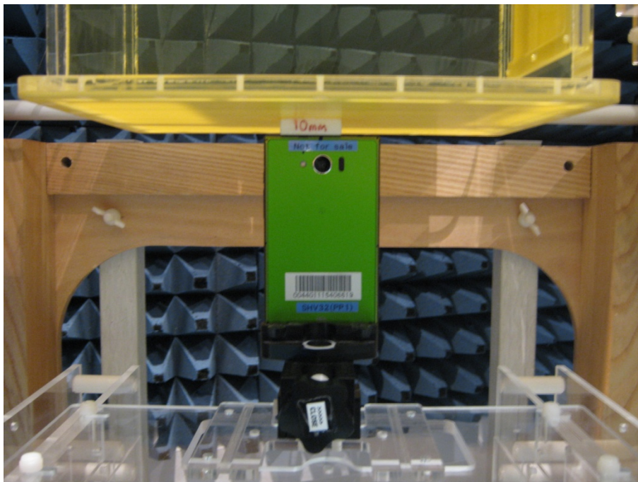
SAR - Top Edge (Body) GSM/WLAN
