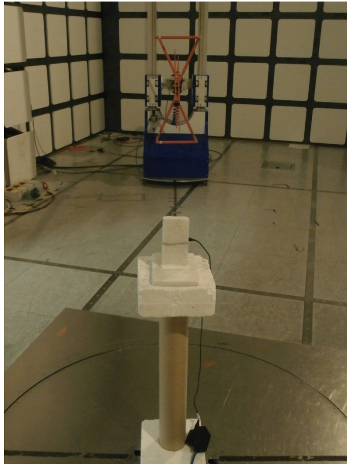
FCC Part 15.247 Radiated Emissions 30 MHz to 1 GHz
