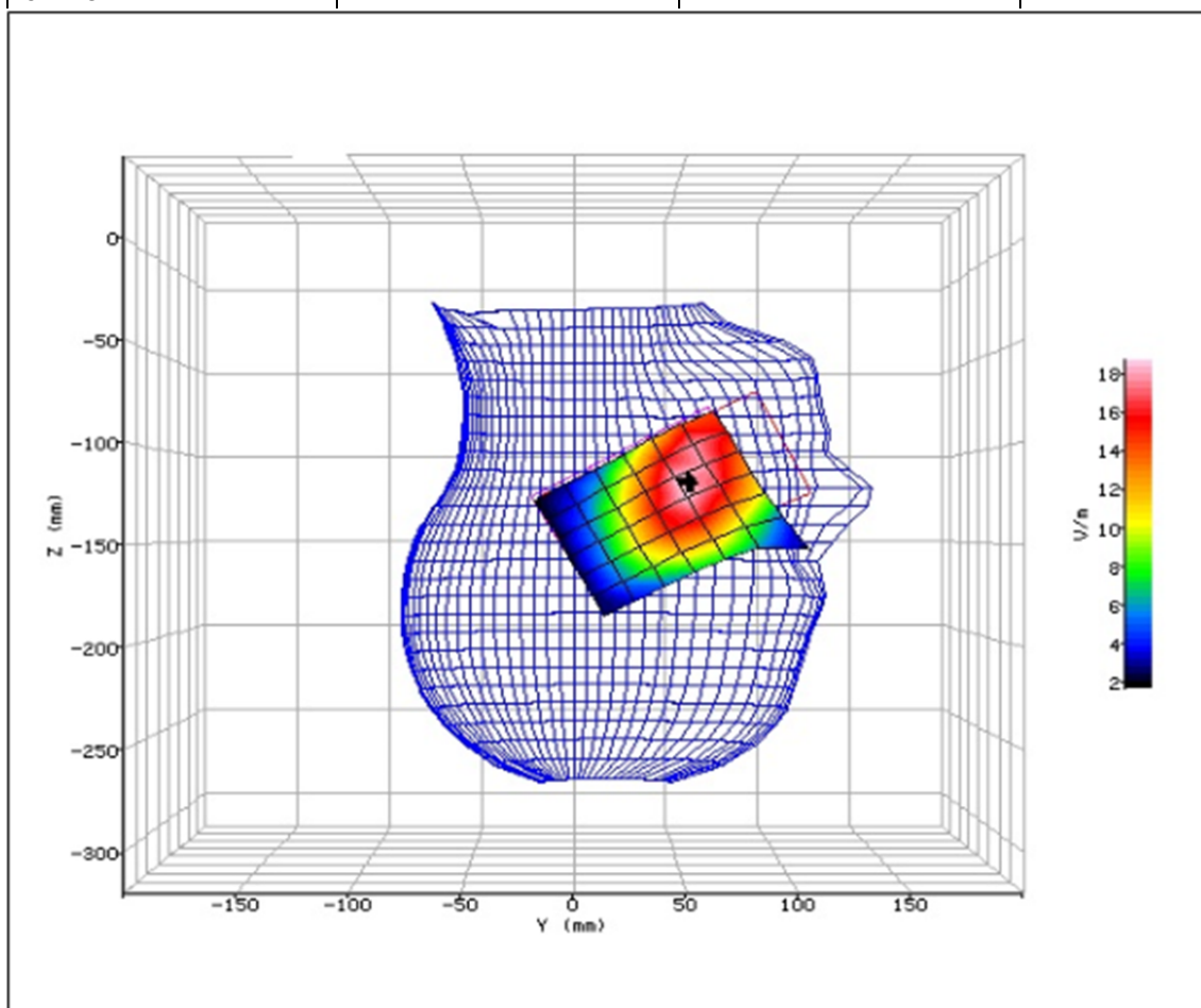
Figure 12: SAR Head Testing Results for the Sharp SHV31 Mobile Handset at 824.2MHz.
