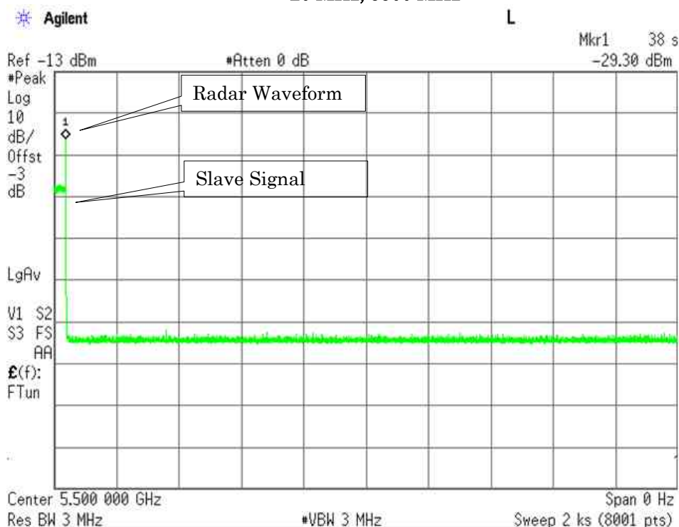
Non-Occupancy Period Plots for 20 MHz, 5500 MHz
