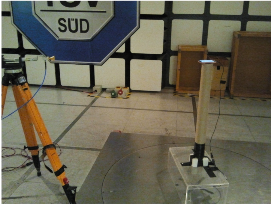
FCC Part 15.247 Radiated Emissions 18GHz-25GHz
