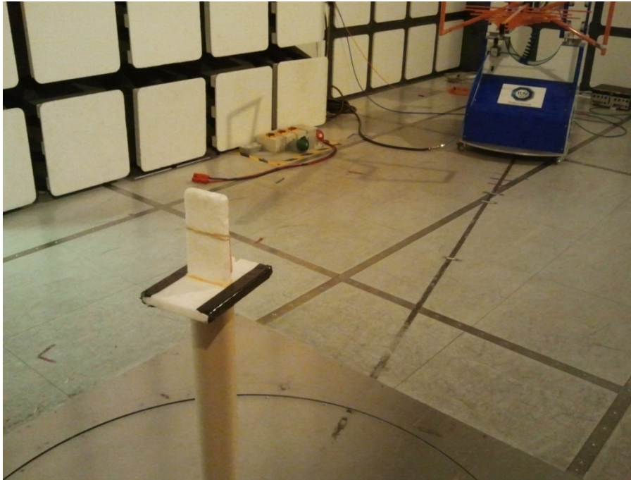
FCC Part 15.247 Radiated Emissions 30MHz-1GHz
