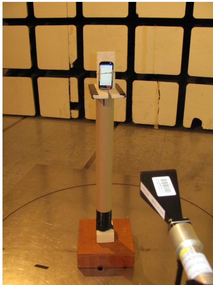
FCC Part 15.407 Radiated Emissions 25GHz-40GHz
