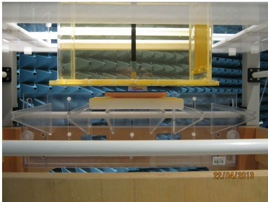
SAR - Body Front Face
