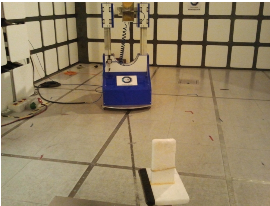
FCC Part 15.247 Radiated Emissions 1GHz-18GHz
