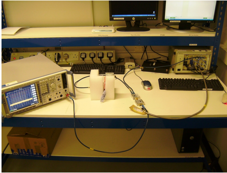
DFS Testing - Calibration Set-Up
