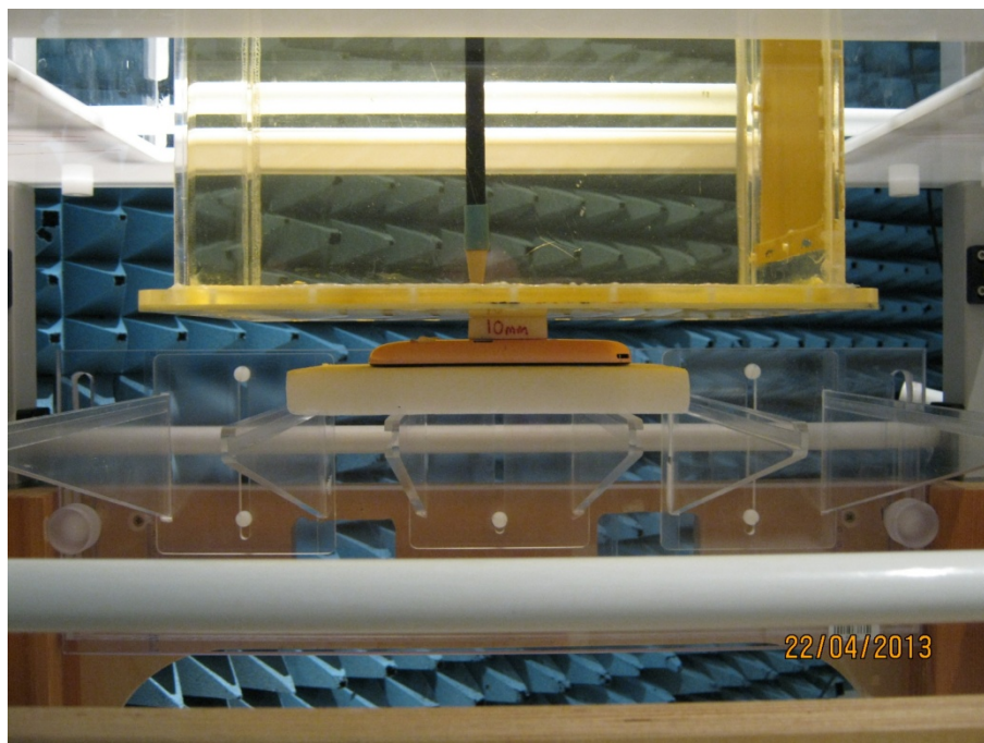
SAR - Body Rear Face
