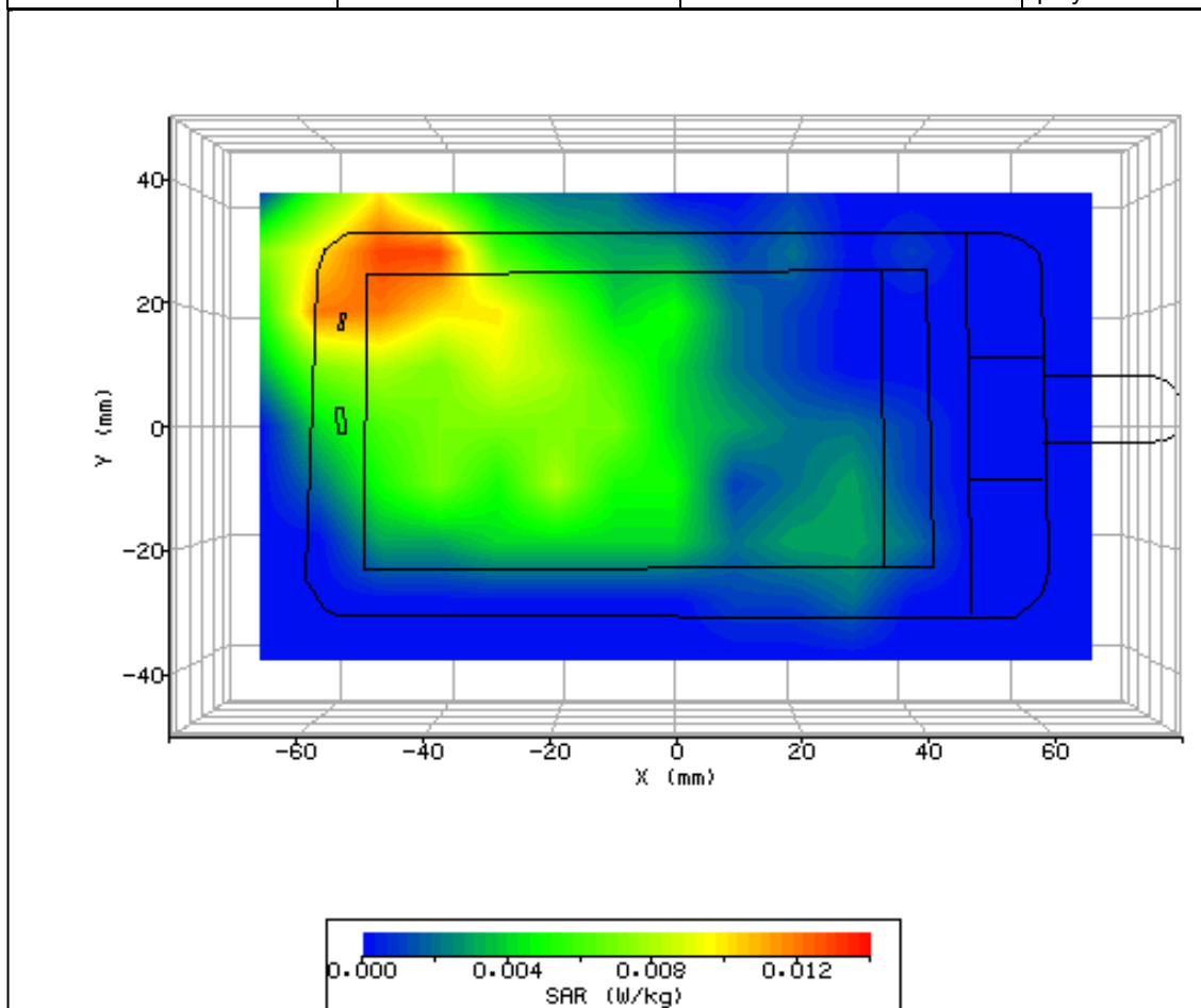
Figure 24: SAR Body Testing Results for the CDMA SHX11 Mobile Handset at 2437.0MHz.
