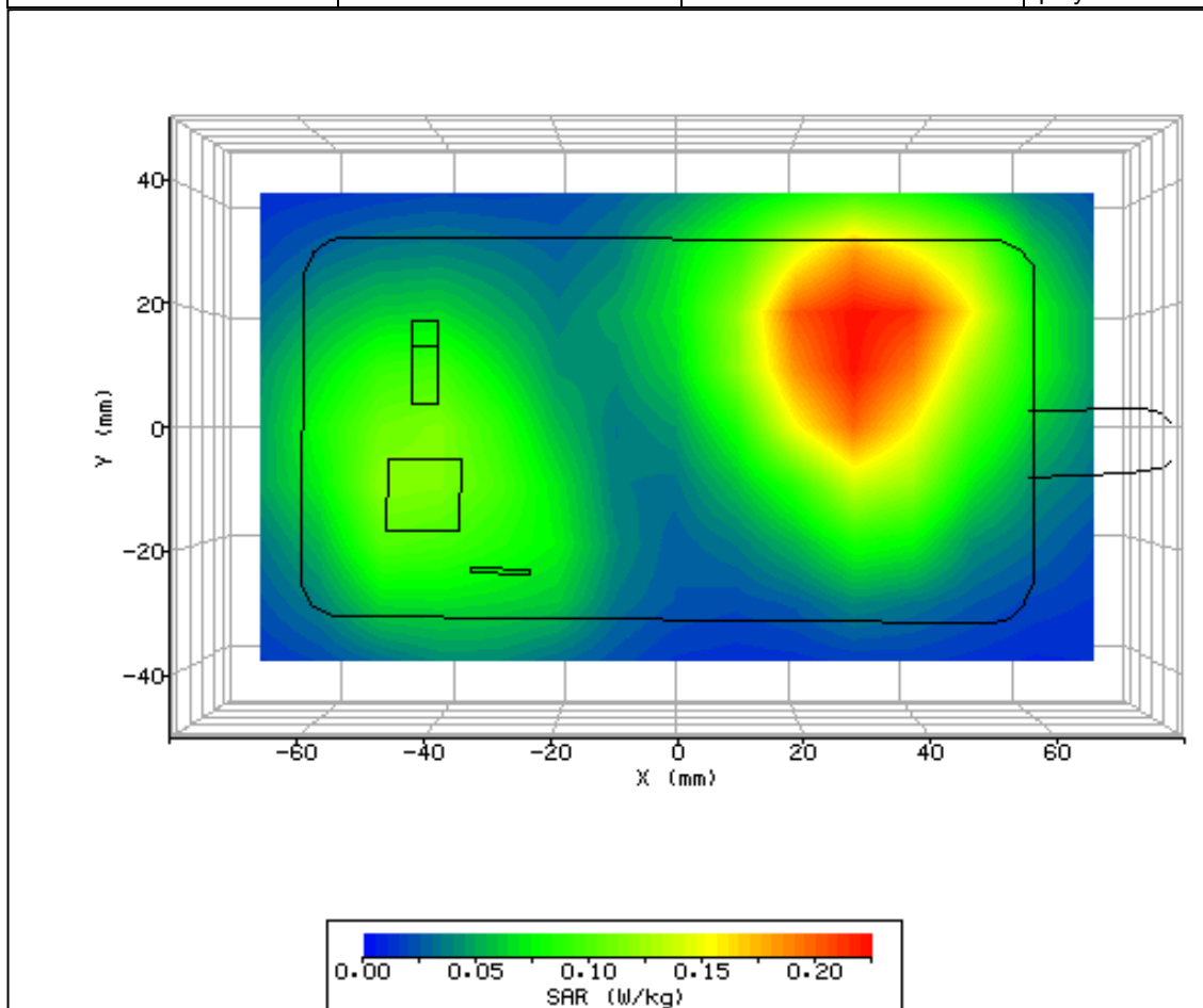
Figure 19: SAR Body Testing Results for the CDMA SHX11 Mobile Handset at 1850.2MHz.
