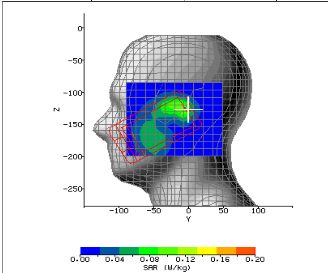
Figure 15: SAR Head Testing Results for the CDMA SHX11 Mobile Handset at 1909.8MHz.
