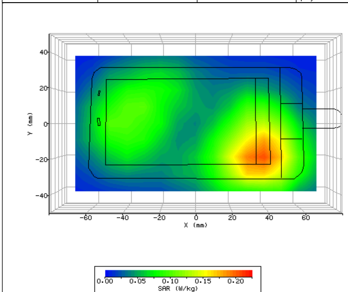
Figure 18: SAR Body Testing Results for the CDMA SHX11 Mobile Handset at 1850.2MHz.
