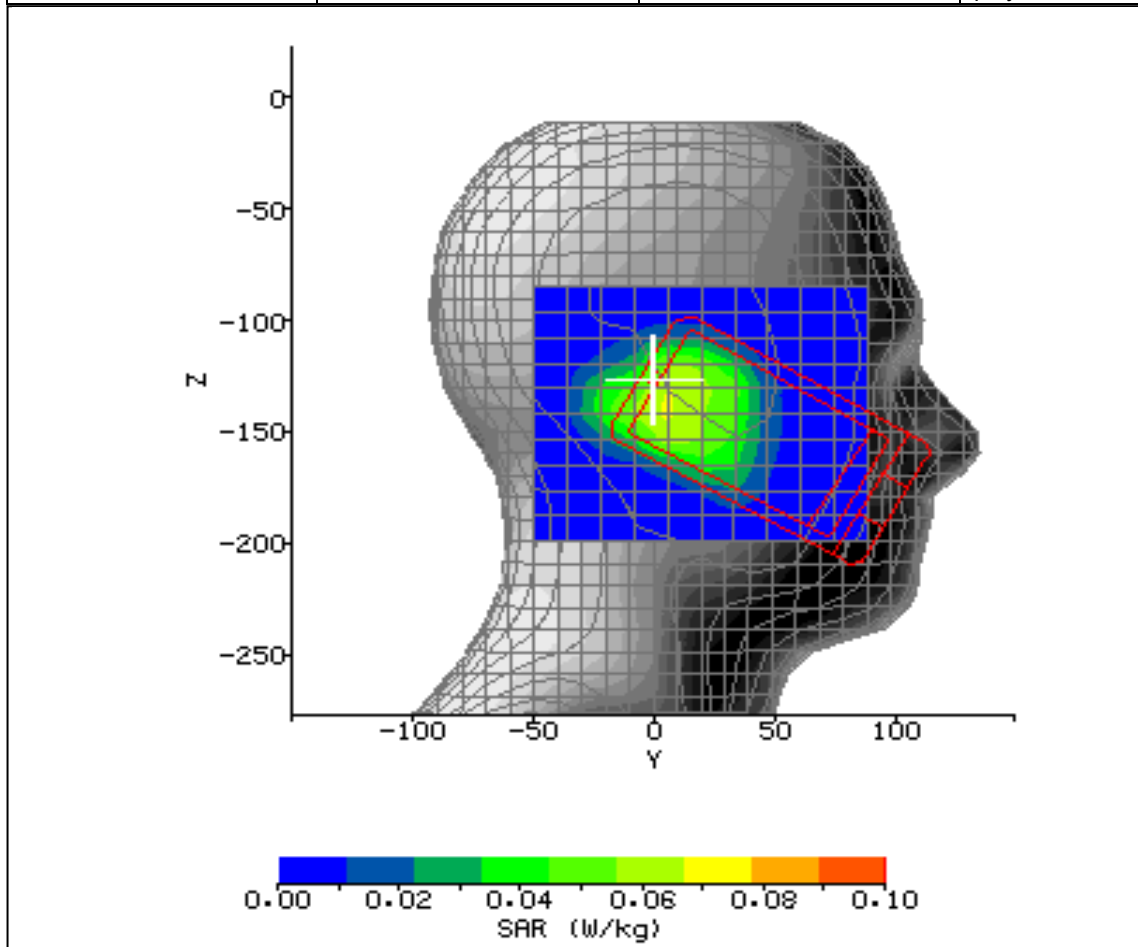
Figure 22: SAR Head Testing Results for the CDMA SHX11 Mobile Handset at 2437.0MHz.
