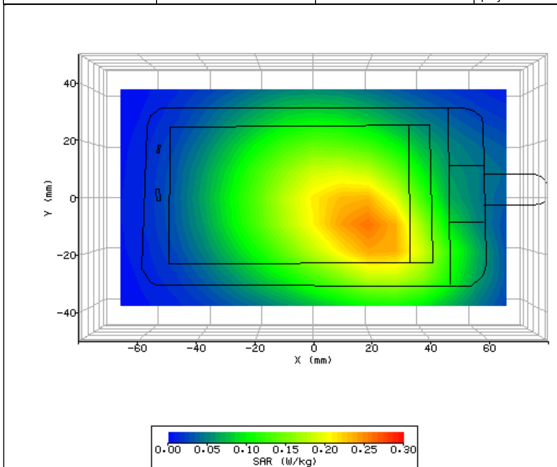
Figure 12: SAR Body Testing Results for the CDMA SHX11 Mobile Handset at 836.52MHz.
