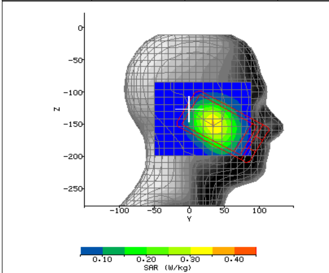
Figure 11: SAR Head Testing Results for the CDMA SHX11 Mobile Handset at 836.52MHz.
