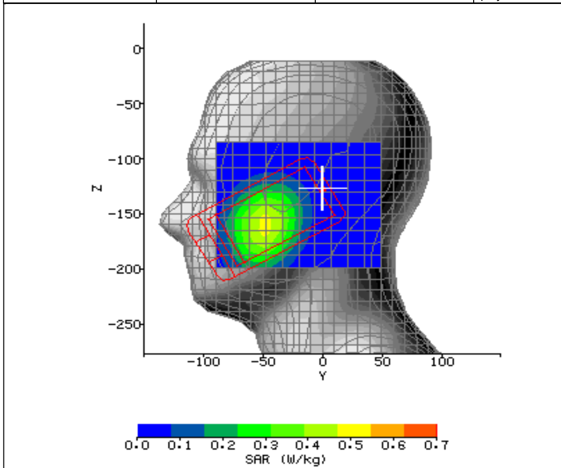
Figure 8: SAR Head Testing Results for the CDMA SHX11 Mobile Handset at 836.52MHz.
