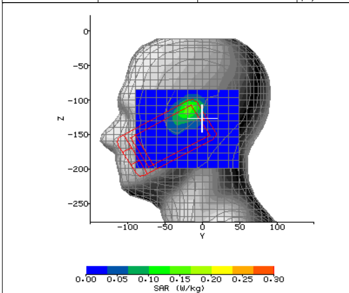
Figure 20: SAR Head Testing Results for the CDMA SHX11 Mobile Handset at 2437.0MHz.
