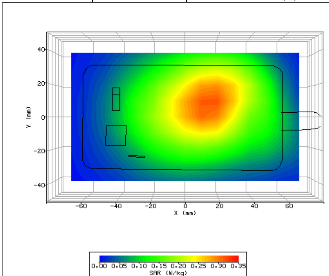
Figure 13: SAR Body Testing Results for the CDMA SHX11 Mobile Handset at 836.52MHz.
