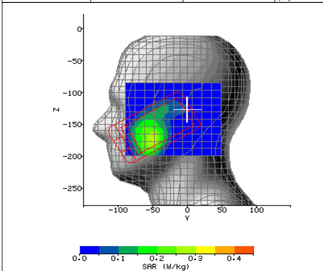
Figure 14: SAR Head Testing Results for the CDMA SHX11 Mobile Handset at 1909.8MHz.
