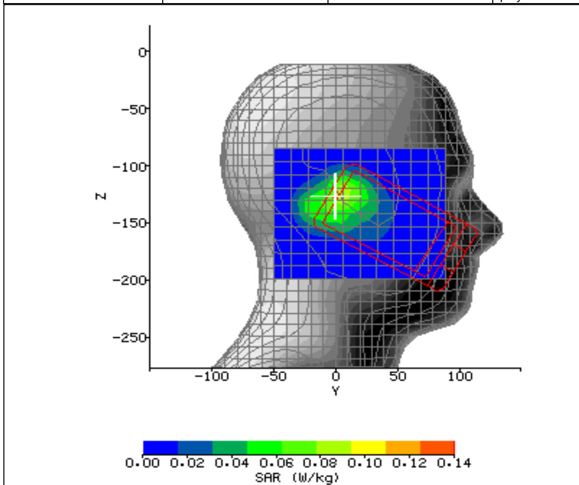
Figure 23: SAR Head Testing Results for the CDMA SHX11 Mobile Handset at 2437.0MHz.
