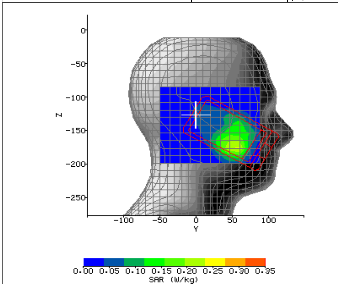
Figure 16: SAR Head Testing Results for the CDMA SHX11 Mobile Handset at 1909.8MHz.
