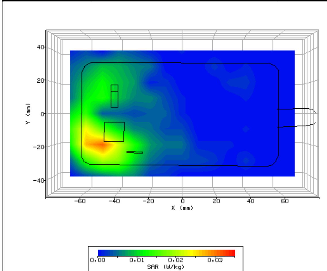
Figure 25: SAR Body Testing Results for the CDMA SHX11 Mobile Handset at 2437.0MHz.
