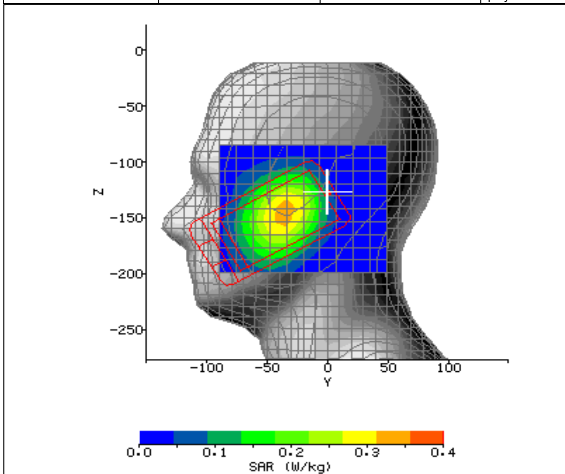
Figure 9: SAR Head Testing Results for the CDMA SHX11 Mobile Handset at 836.52MHz.
