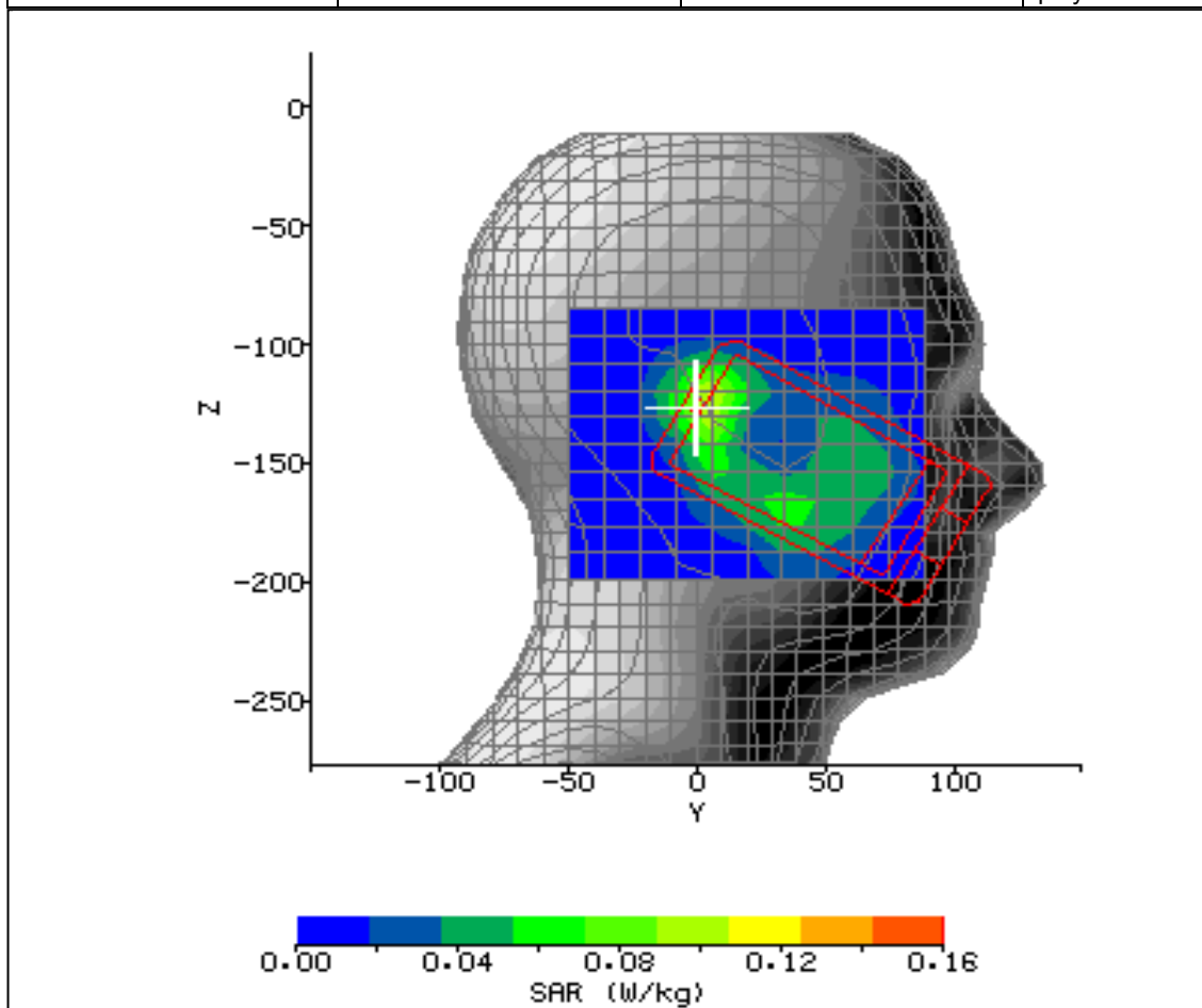
Figure 17: SAR Head Testing Results for the CDMA SHX11 Mobile Handset at 1909.8MHz.
