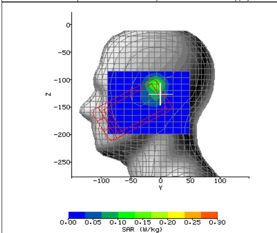
Figure 21: SAR Head Testing Results for the CDMA SHX11 Mobile Handset at 2437.0MHz.
