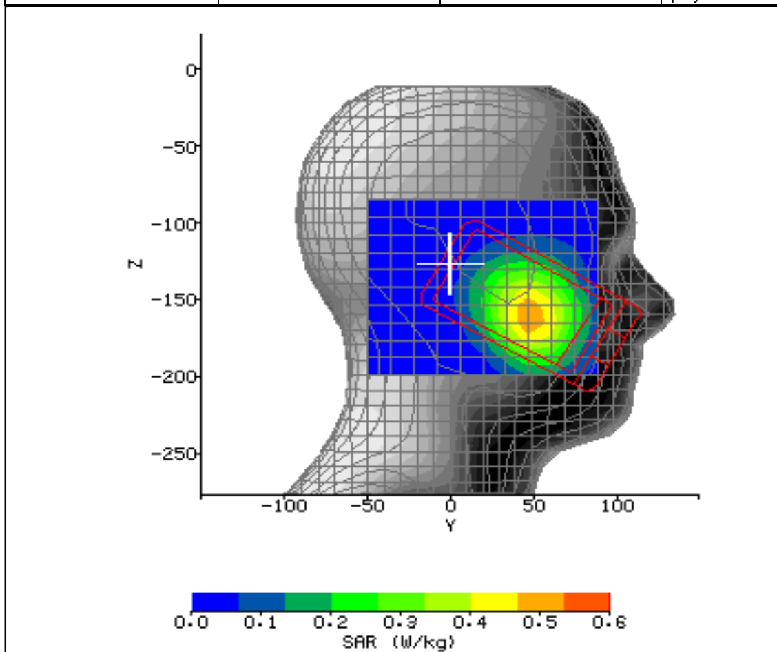
Figure 10: SAR Head Testing Results for the CDMA SHX11 Mobile Handset at 836.52MHz.
