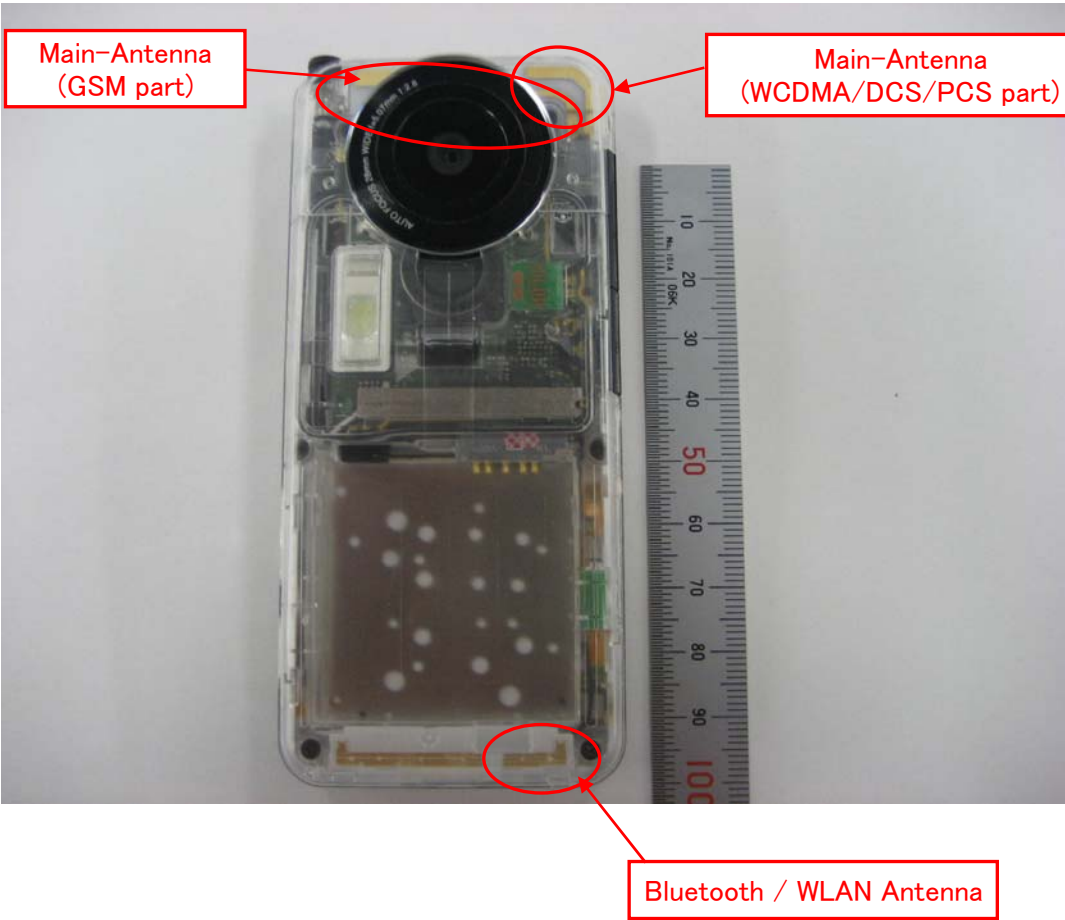
Distance between PCS antenna and Bluetooth / WLAN antenna
