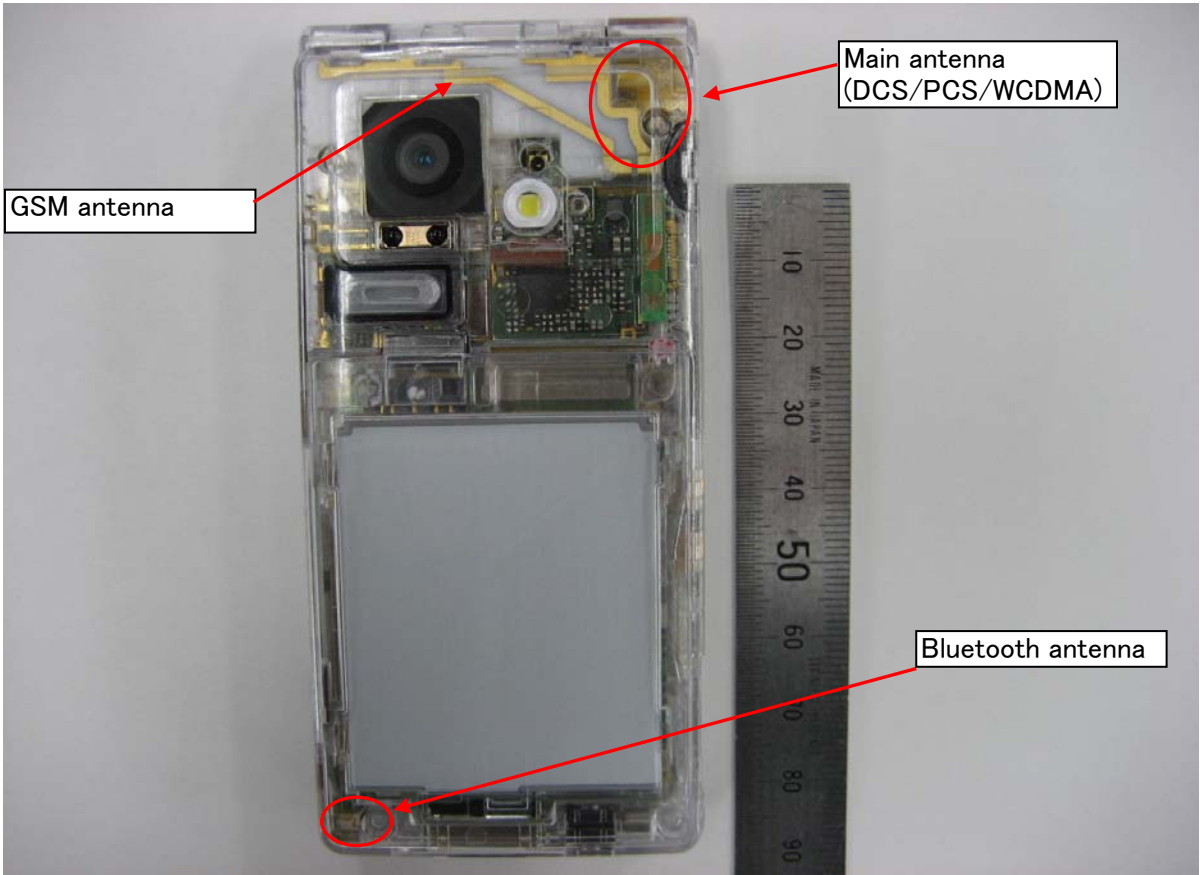
Distance between PCS antenna and Bluetooth antenna
