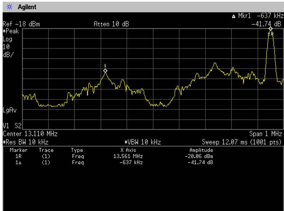
Band-Edge Emission
