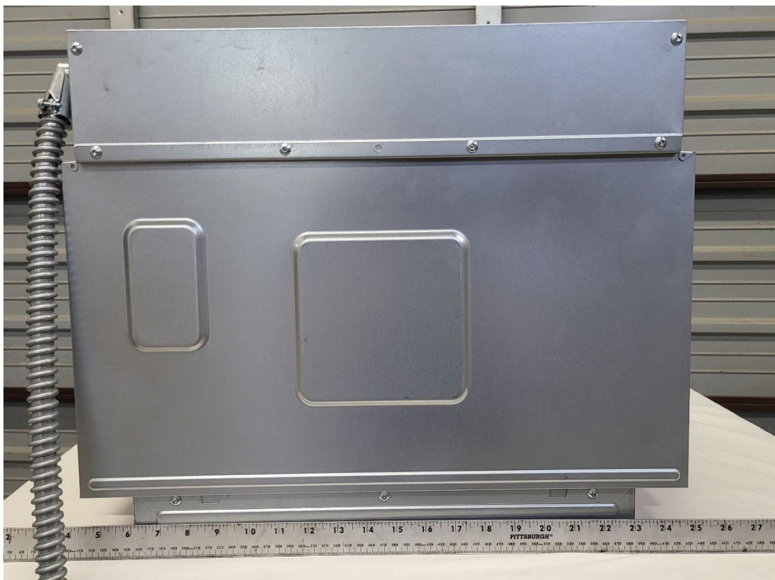
Figure 3. EUT Back
