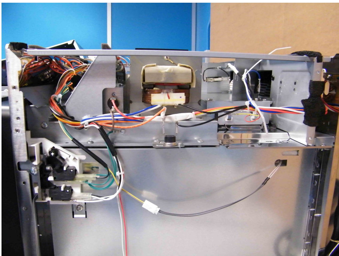
RIGHT SIDE WITH OUTER COVER REMOVED
