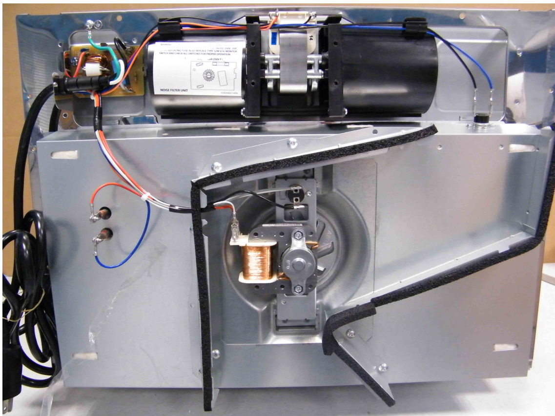
REAR VIEW WITH COVER REMOVED SHOWING NOISE FILTER UNIT, COOLING FAN MOTOR AND CONVECTION FAN MOTOR
