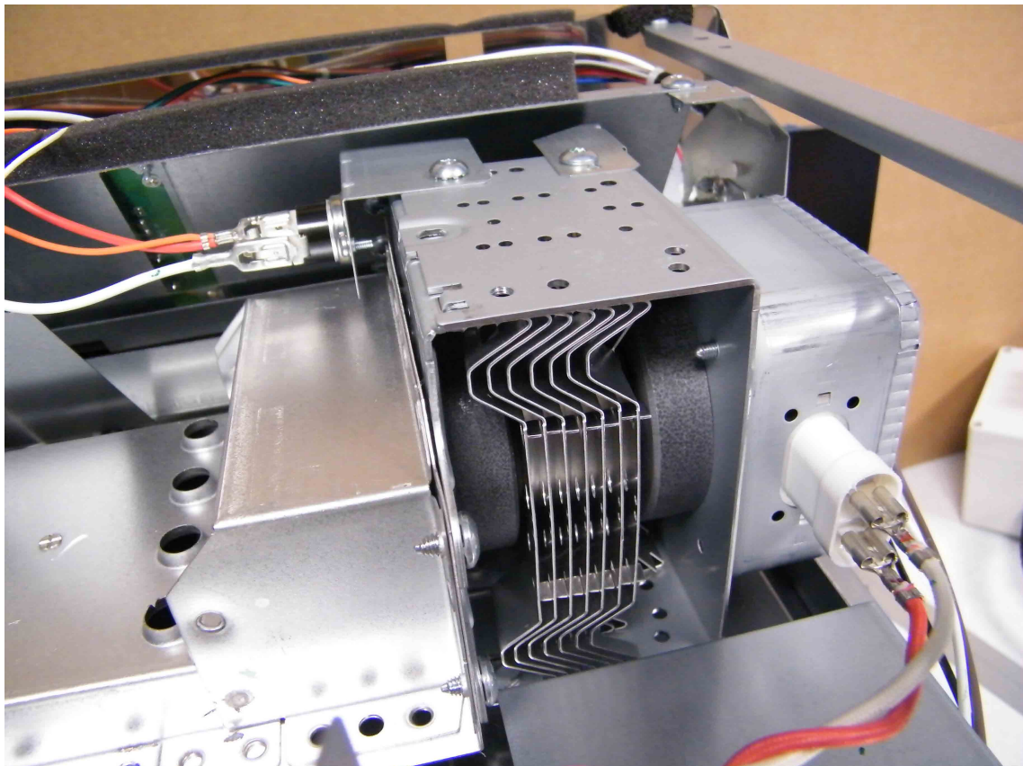
MAGNETRON AND PROTECTIVE THERMAL CUT-OUT
