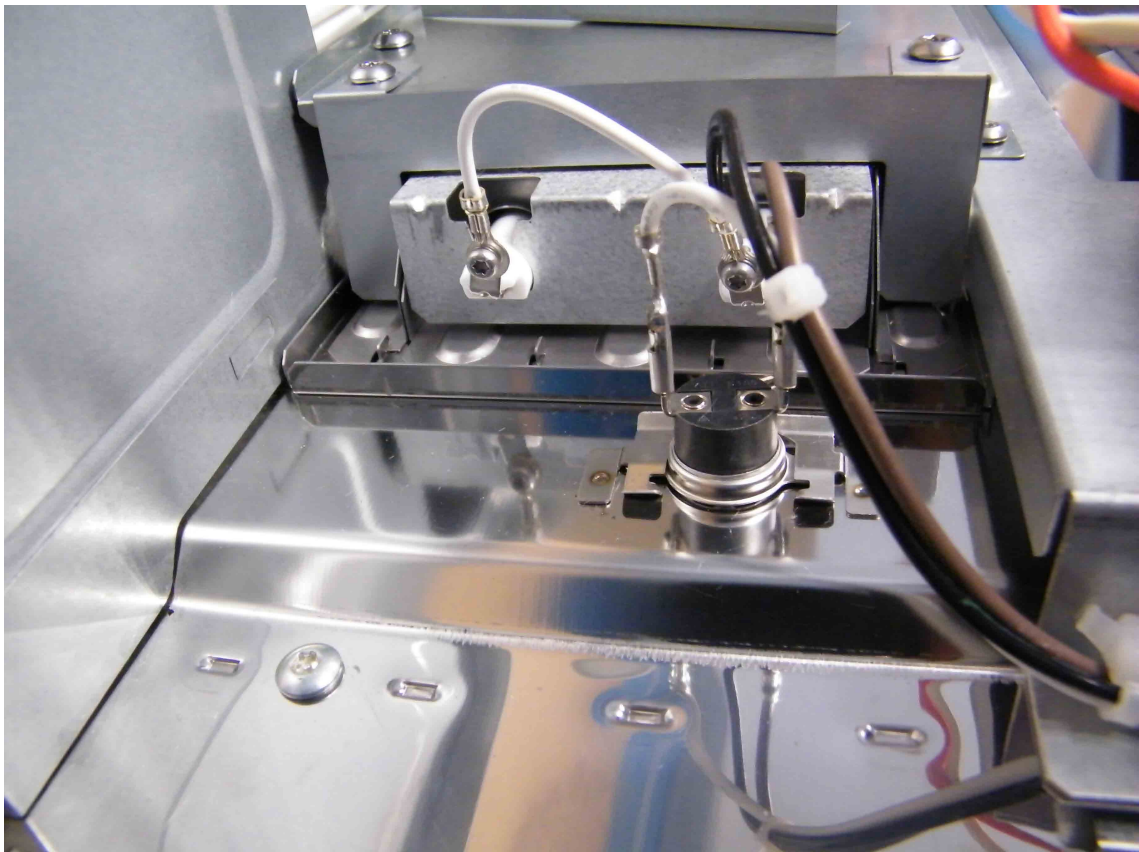
GRILL HARNESS - LEFT SIDE
