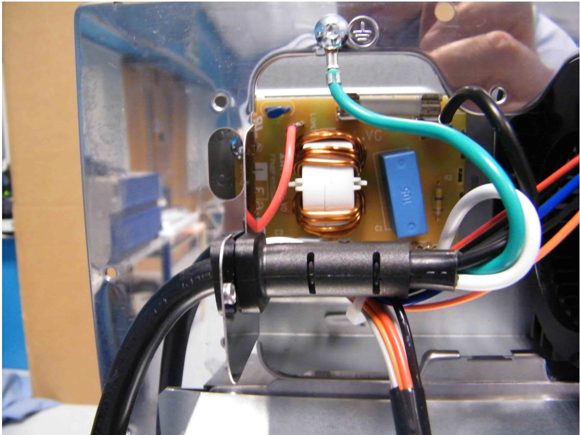
NOISE FILTER UNIT AND POWER CORD
