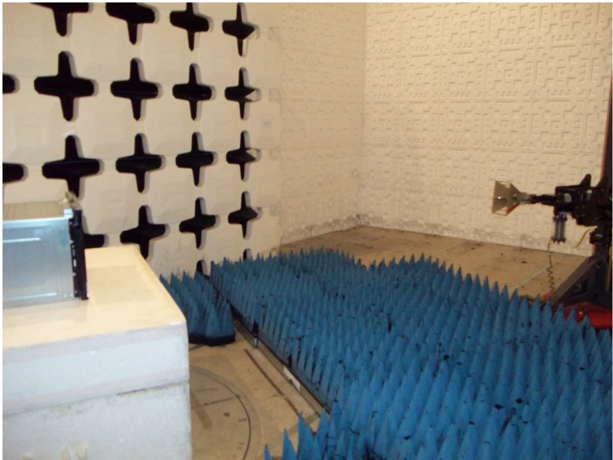
Figure 4. Radiated Emissions Measurement, above 1000 MHz and Variation in Operating Frequency
