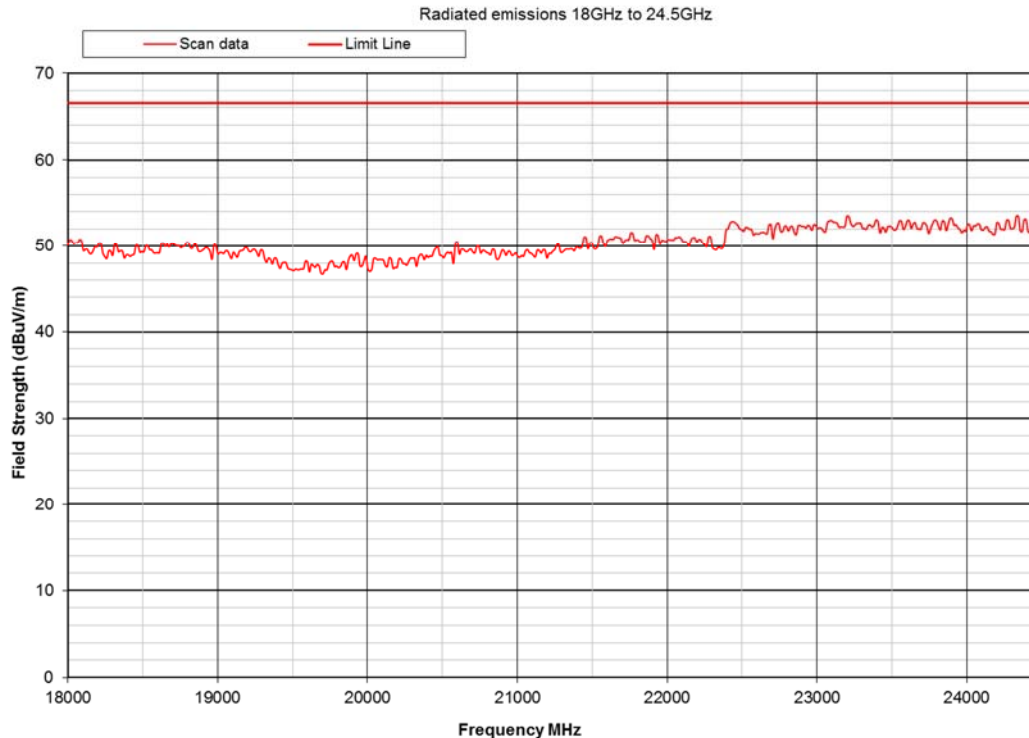
Figure 5.5.5 Radiated emissions results Antenna Vertical (Chamber measurement at 3m, 18GHz to 24.5GHz Peak data-Information only)
