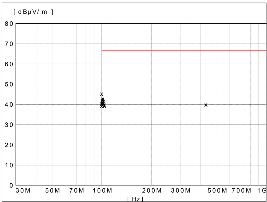
Figure 5.5.2 Radiated emissions results (R02, OATS) – Maximised Quasi Peak data.
