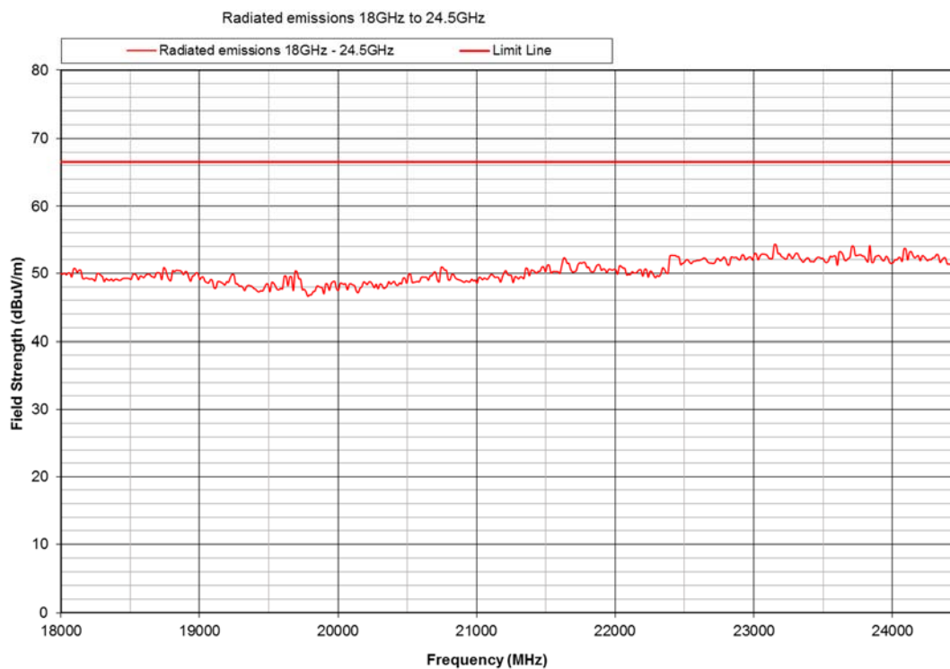
Figure 5.5.4 Radiated emissions results Antenna Horizontal (Chamber measurement at 3m, 18GHz to 24.5GHz Peak data-Information only)
