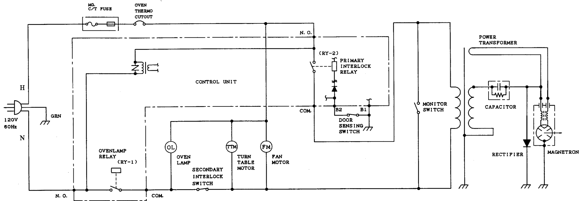
SCHEMATIC DIAGRAM (DOOR CLOSED, COOK OFF CONDITION)
