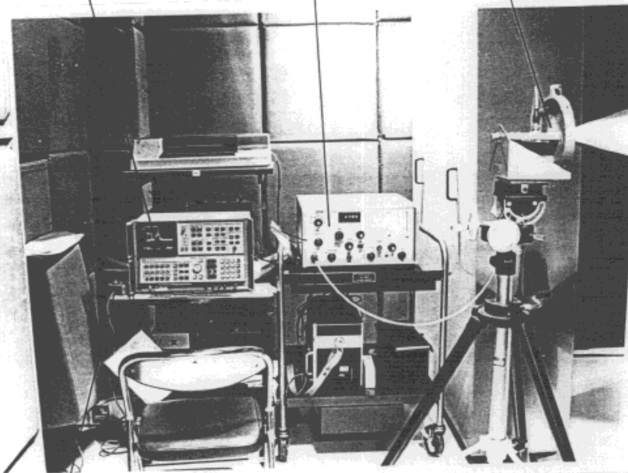
Spectrum Analyzer 8566B
