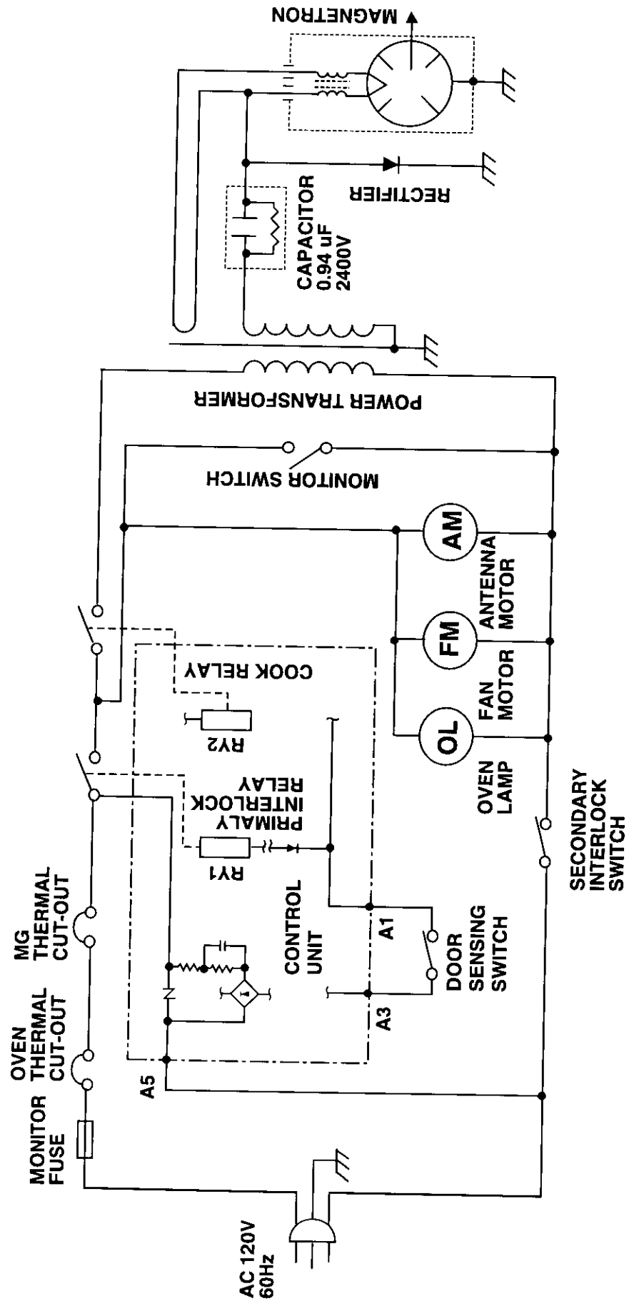
SCHEMATIC DIAGRAM (DOOR CLOSED, COOK OFF CONDITION)
