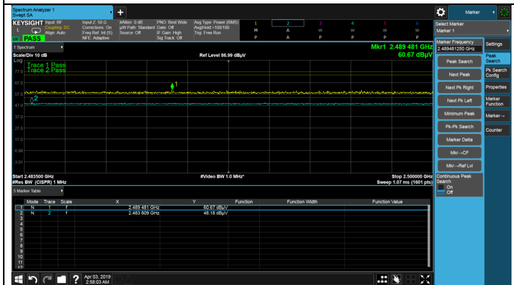
BLE-2480MHz
