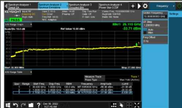
Channel 41515 (2682.5MHz)
