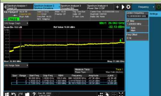
Channel 41490 (2680MHz)
