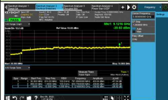
Channel 27025 (847.5MHz)
