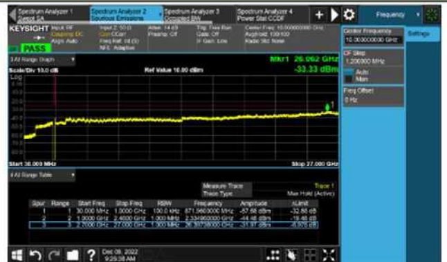
Channel 40620 (2593MHz)
