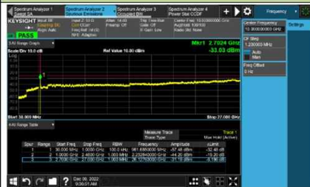
Channel 41515 (2682.5MHz)
