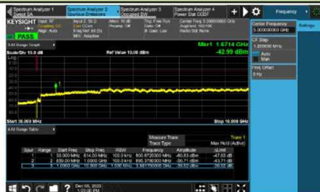
Channel 26915 (836.5MHz)
