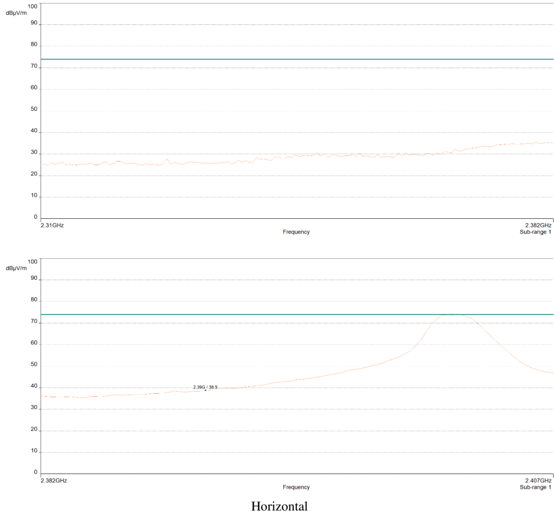
Plot 18: Radiated Band Edge, Low Channel 2402MHz, Peak
