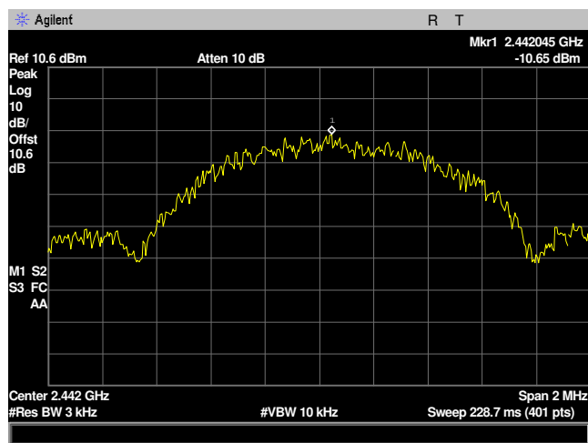
Plot 33: Peak Power Spectral Density, 2442MHz Mid Channel
