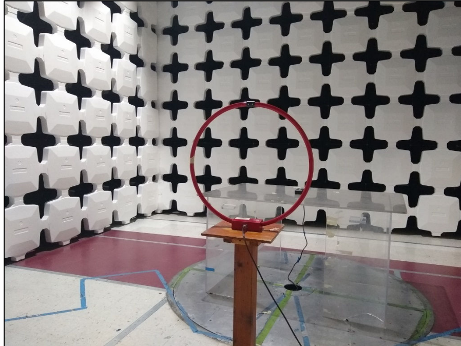
Photograph 5. Radiated Spurious Emissions, Substitution Method Below 30MHz, Test Setup
