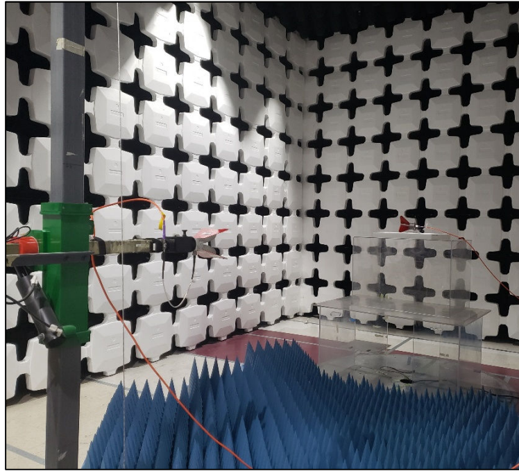
Photograph 3. Radiated Spurious Emissions, Substitution Method Above 1GHz, Test Setup
