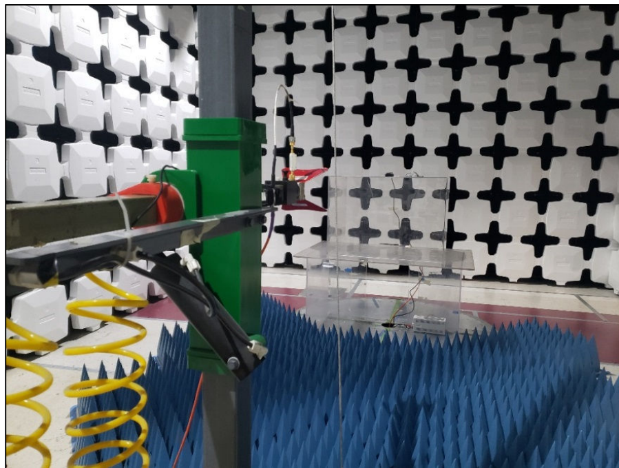
Photograph 2. Radiated Emissions, 1GHz – 18 GHz, Test Setup
