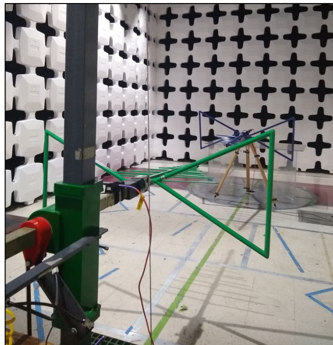
Photograph 4. Radiated Spurious Emissions, Substitution Method Below 1GHz, Test Setup
