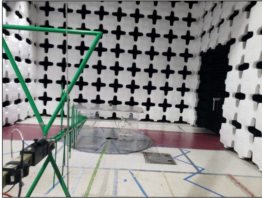
Photograph 1. Radiated Emissions, 30 MHz – 1 GHz, Test Setup
