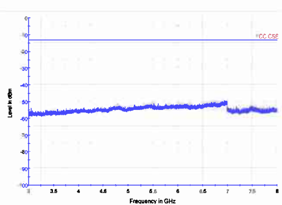
LTE Band 13 5MHz CH-High 3GHz~8GHz
