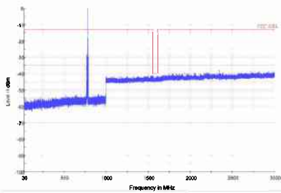
LTE Band 13 5MHz CH-Low 30MHz~3GHz
