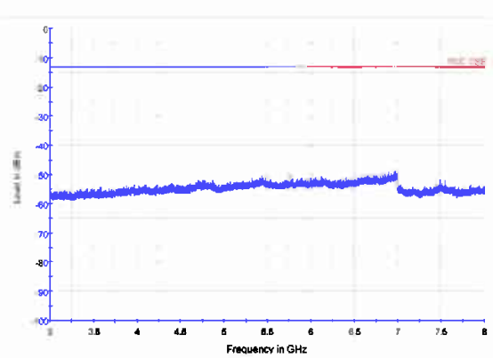
LTE Band 13 5MHz CH-Middle 3GHz~8GHz
