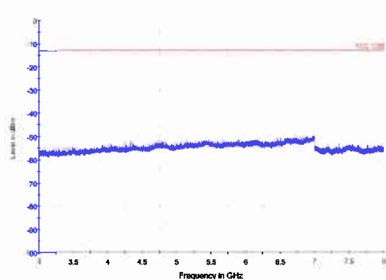
LTE Band 12 5MHz CH-High 3GHz~8GHz
