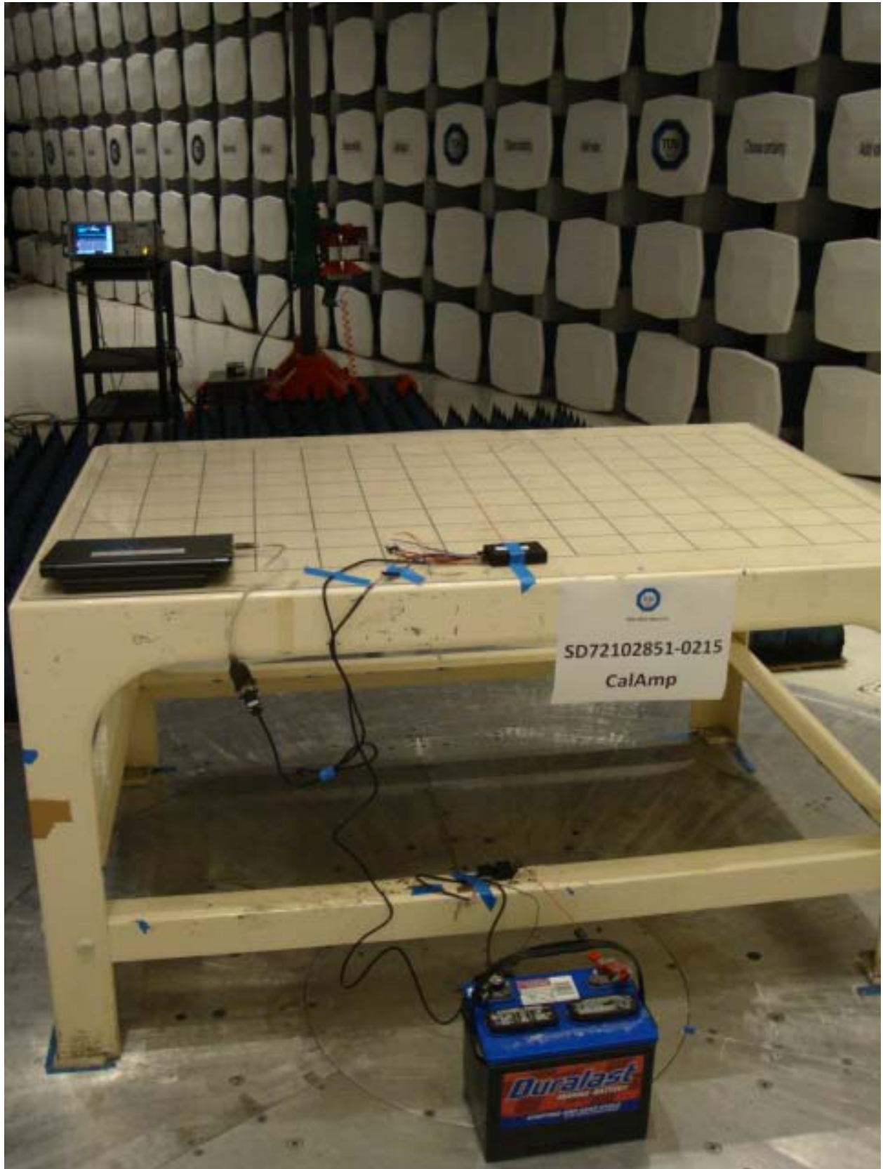
Radiated Emissions Test Setup (above 1GHz)
