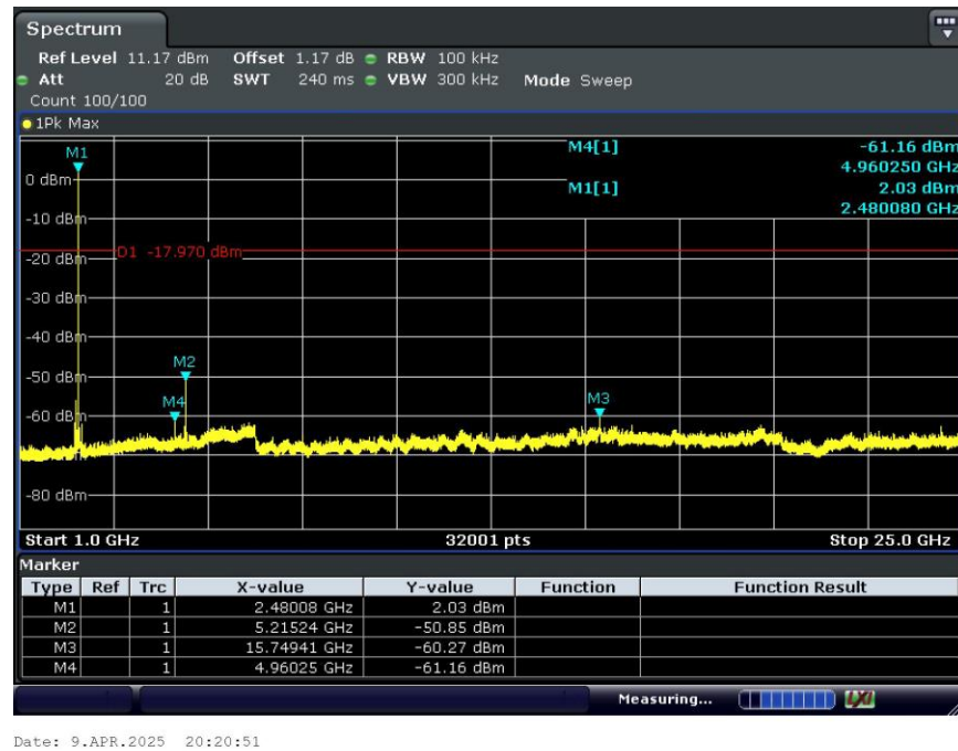
Figure 19. Conducted Emissions, Conducted Spurious Emissions: High Channel, 2480 MHz Plot
