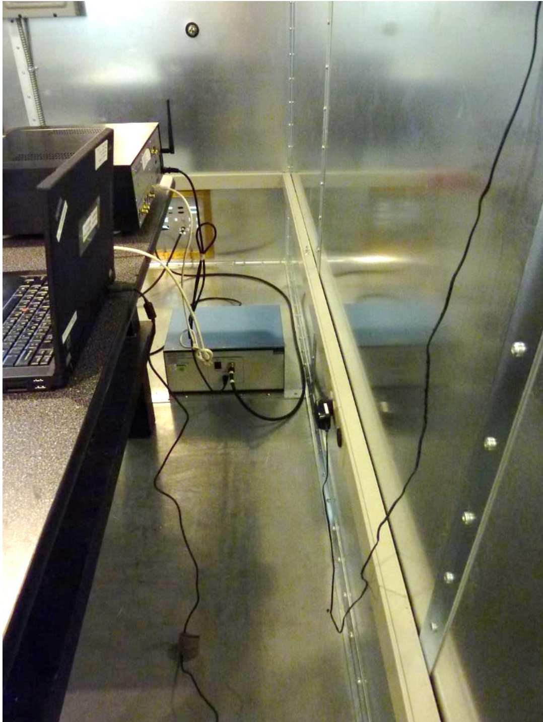
Figure 11: Conducted Emission Test Setup (Side)
