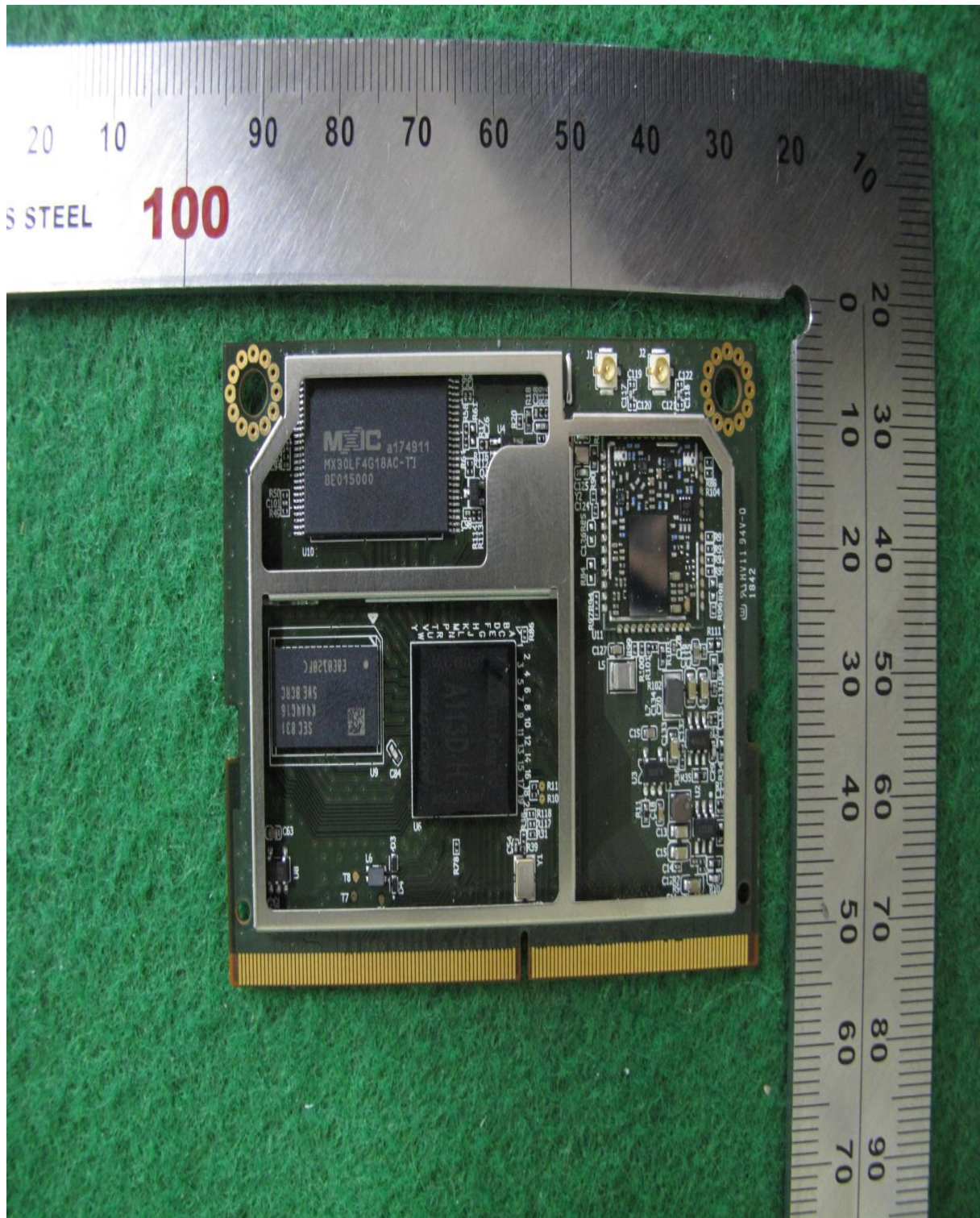
Internal View of EUT without shield can
