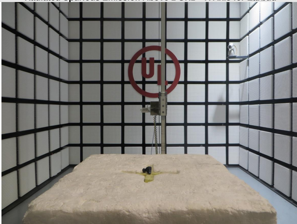
Radiated Spurious Emission Above 1 GHz – X Axis for Earbud
