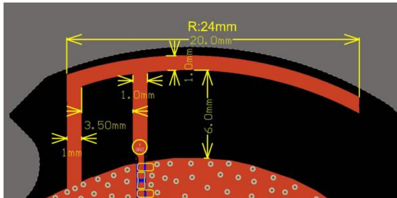
Figure 1 Antenna
