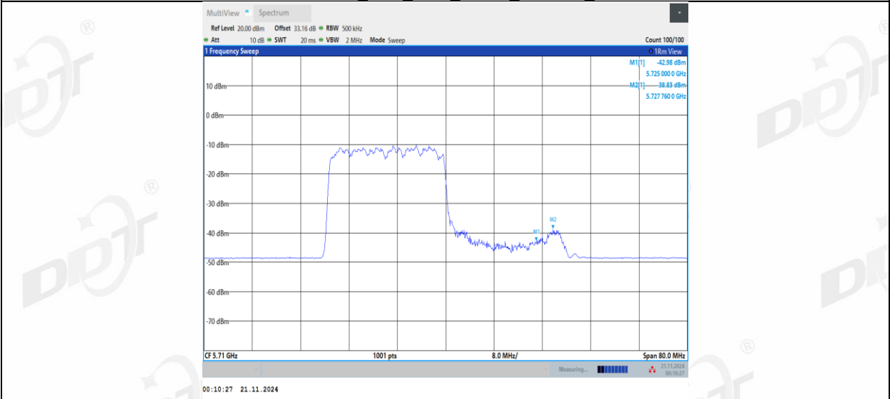
11AX40MIMO Ant2 5710 UNII-3 242Tone RU62
