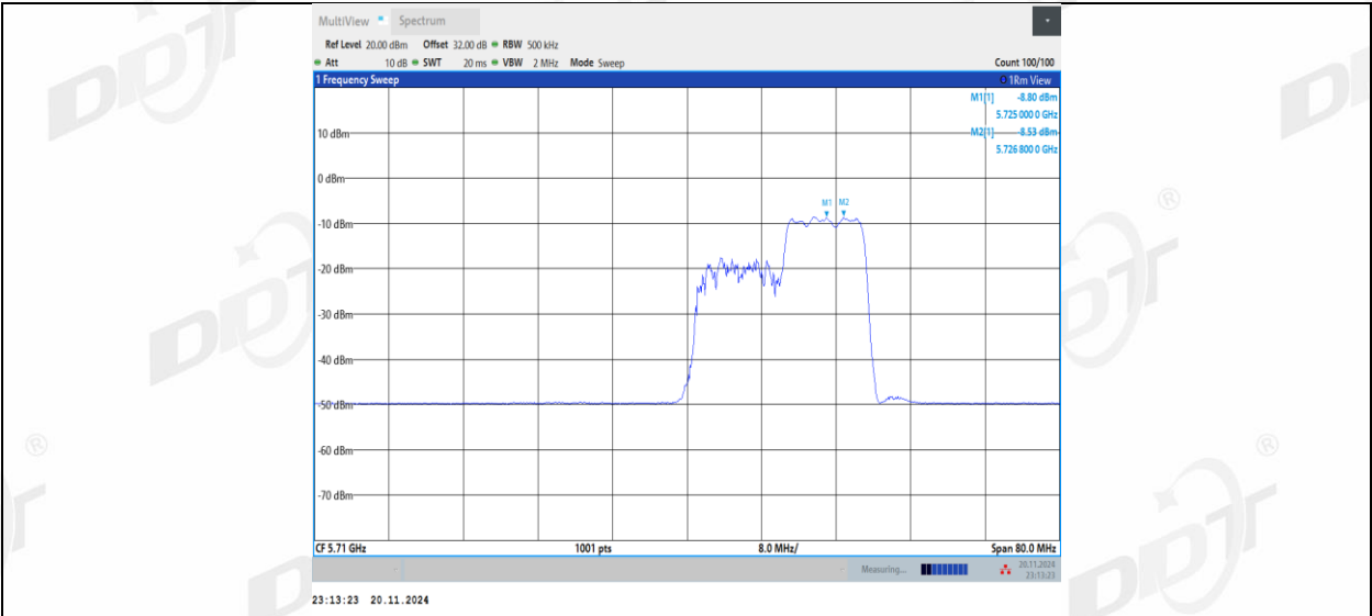
11AX40MIMO Ant2 5710 UNII-3 242Tone RU61
