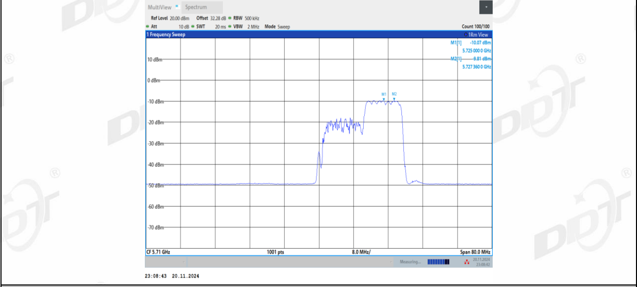
11AX40MIMO Ant1 5710 UNII-3_242Tone RU61
