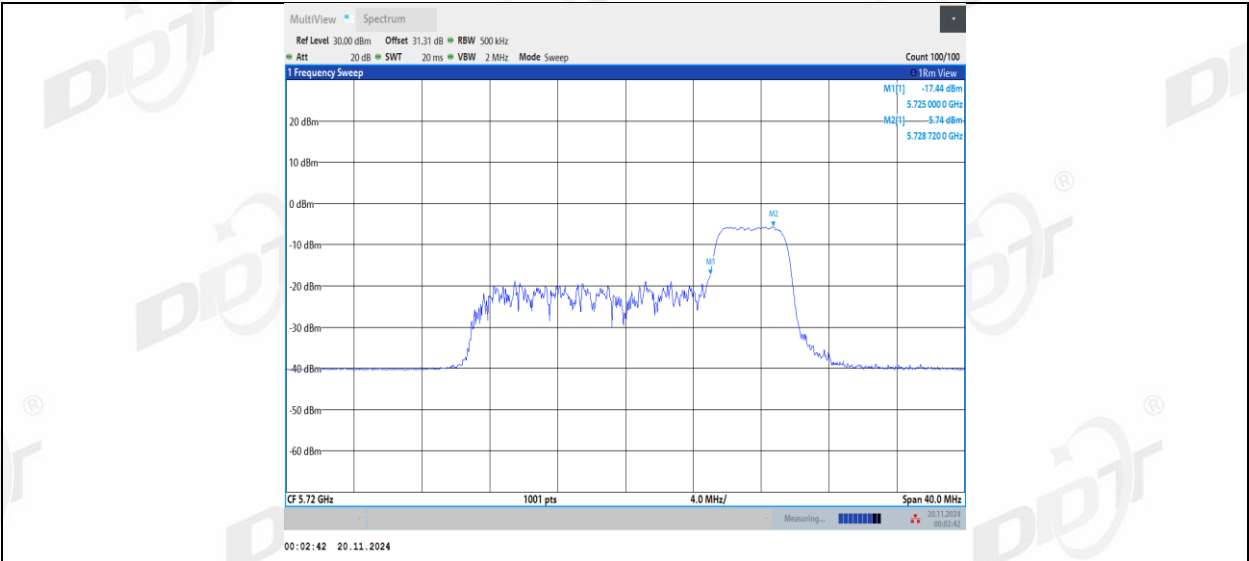
11AX20MIMO Ant1 5720 UNII-3 106Tone RU53
