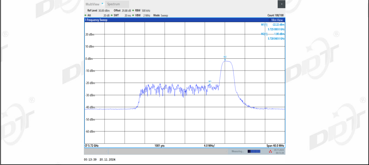
11AX20MIMO Ant2 5720 UNII-3 52Tone RU37
