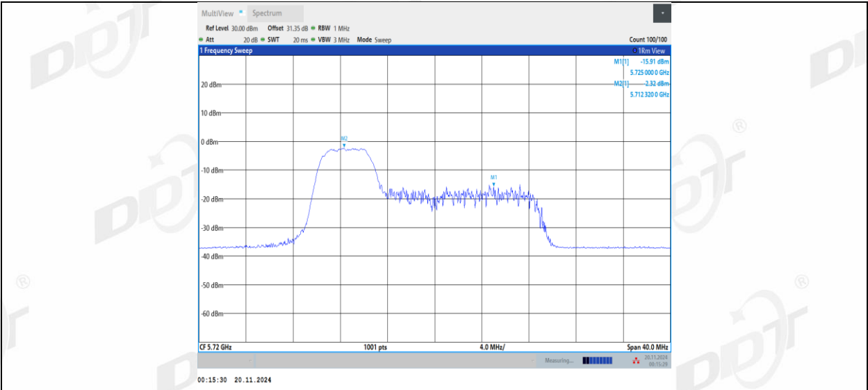
11AX20MIMO Ant2_5720 UNII-2C_52Tone_RU38
