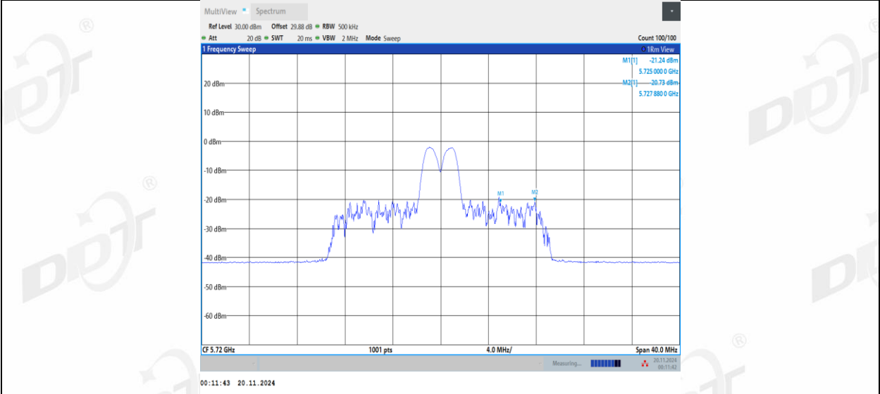
11AX20MIMO Ant2 5720 UNII-3 26Tone RU8
