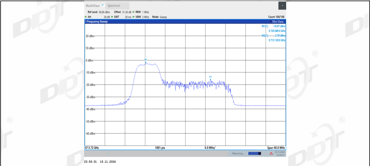
11AX20MIMO Ant1_5720 UNII-2C_52Tone_RU38
