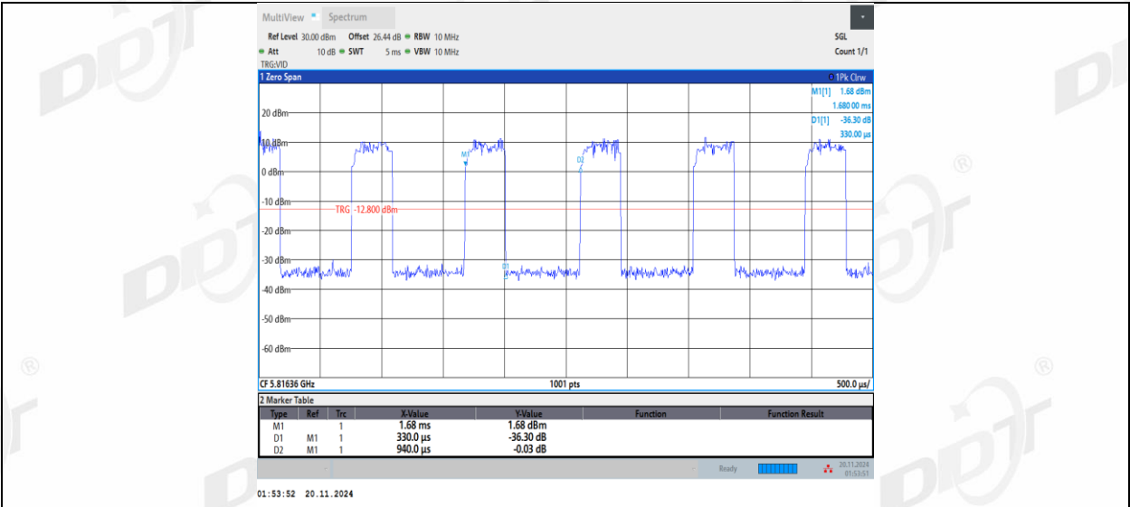
11AX20MIMO Ant2_5825_52Tone_RU38
