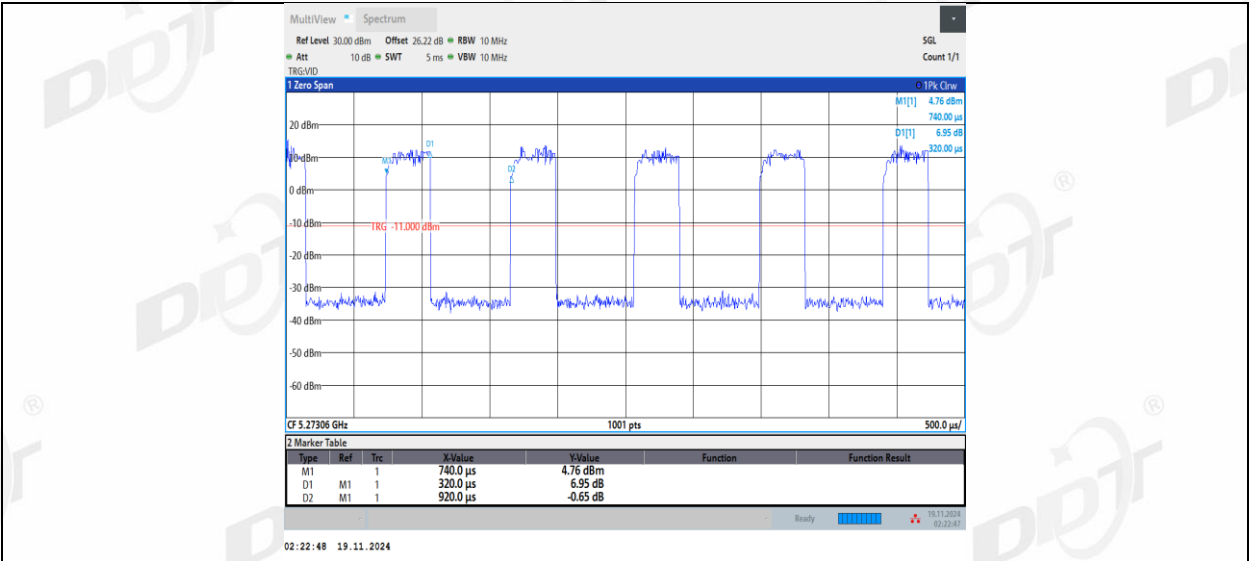
11AX20MIMO Ant2_5280_52Tone_RU38
