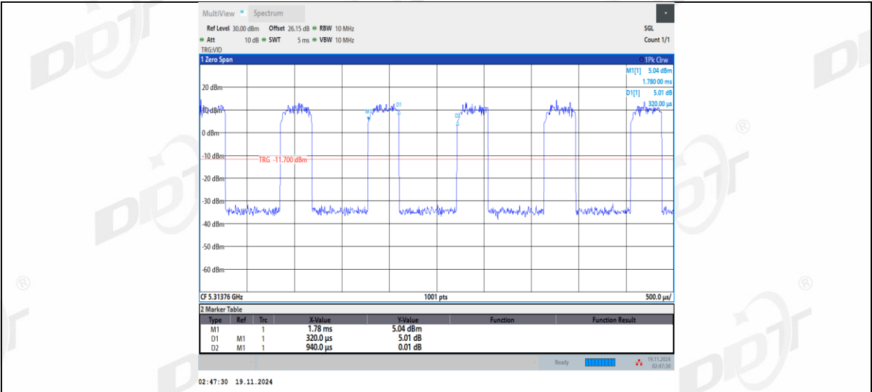
11AX20MIMO Ant2_5320_52Tone_RU38
