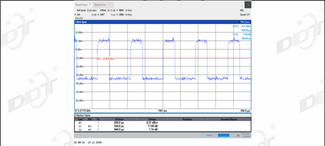
11AX20MIMO Ant2_5320_52Tone_RU39
