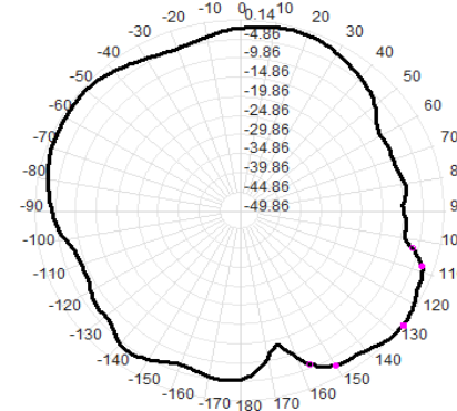
2460.0MHz Total(E1), Max= -0.11dBi
